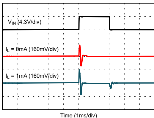
图 6-29. Line Transient Response ( V_{REF} = 1.25\text{V} , C_L = 1\mu\text{F} )
