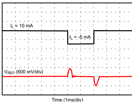
图 6-25. Load Transient Response ( V_{REF} = 2.5\text{V} , C_L = 1\mu\text{F} )
