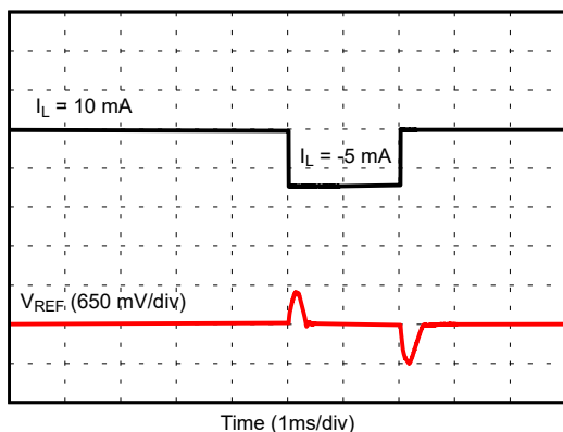
图 6-27. Load Transient Response ( V_{REF} = 1.25\text{V} , C_L = 1\mu\text{F} )
