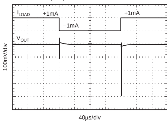
LOAD TRANSIENT C_L = 0\text{ pF} , \pm 1\text{ mA} OUTPUT PULSE
