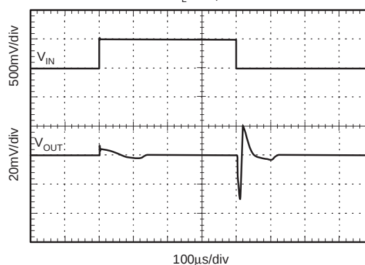
LOAD TRANSIENT C_L = 1\mu\text{F} , \pm 10\text{ mA} OUTPUT PULSE
