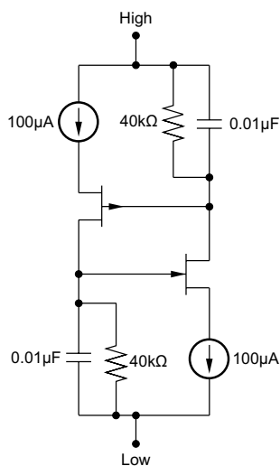
(c) Floating 200µA cascoded current source.
