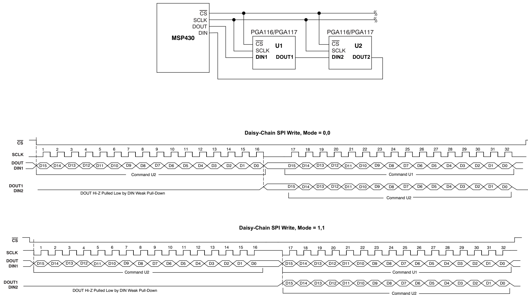
Figure 63. SPI Daisy-Chain Write Timing Diagrams
