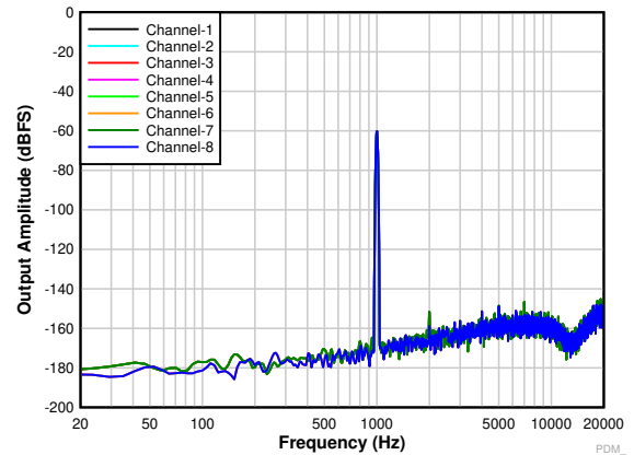
PDMCLKx = 3.072MHz 的五阶 PDM 调制器
