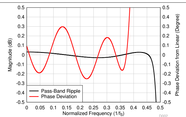
图 7-48. Low-Latency Decimation Filter Pass-Band Ripple and Phase Deviation
