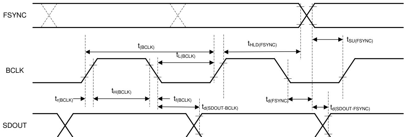
图 6-2. TDM (With BCLK_POL = 1), I²S, and LJ Interface Timing Diagram
