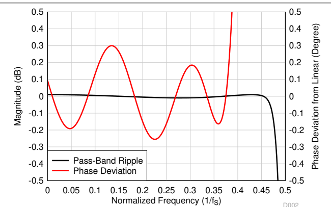
图 7-40. Low-Latency Decimation Filter Pass-Band Ripple and Phase Deviation
