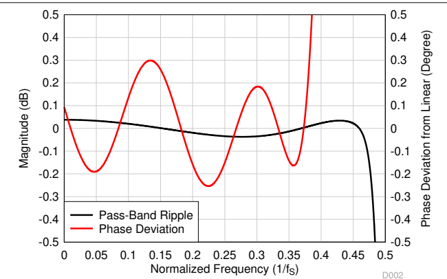
图 7-46. Low-Latency Decimation Filter Pass-Band Ripple and Phase Deviation
