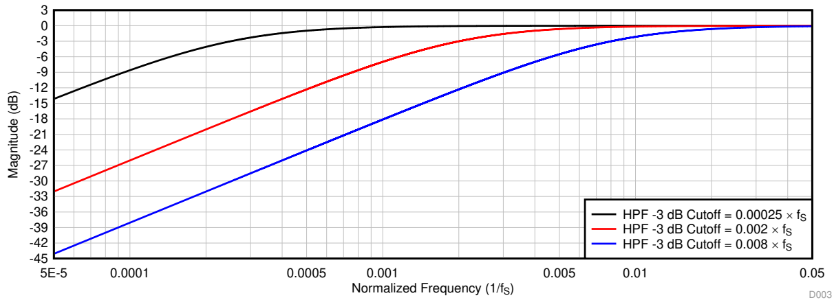
图 42. HPF Filter Frequency Response Plot
