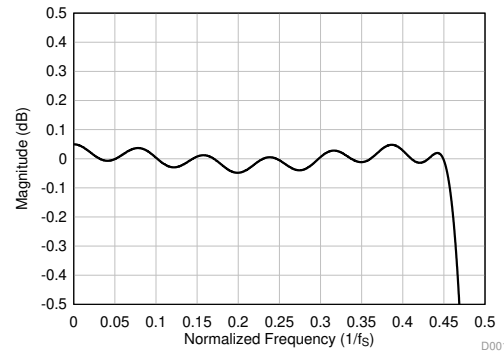
图 55. Linear Phase Decimation Filter Pass-Band Ripple
