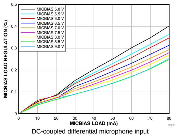
图 18. MICBIAS Load Regulation vs MICBIAS Load Current
