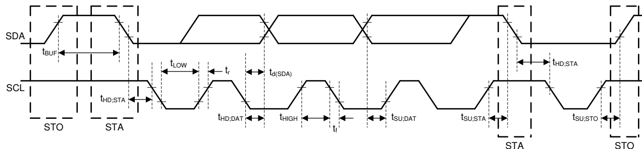
图 1. I²C Interface Timing Diagram
