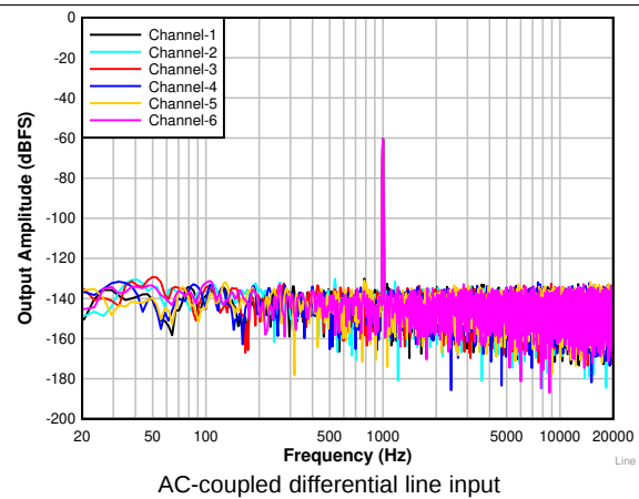
图 9. FFT With a -60-dBr Input
