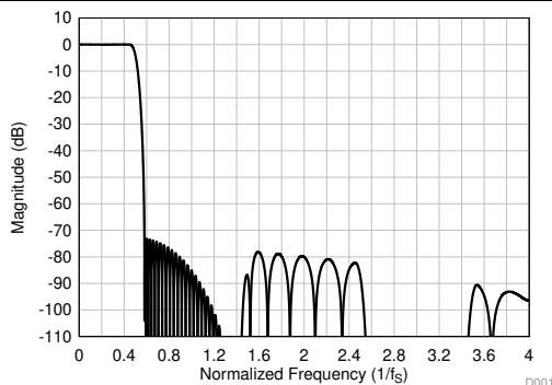
图 48. Linear Phase Decimation Filter Magnitude Response
