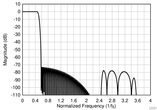
图 46. Linear Phase Decimation Filter Magnitude Response
