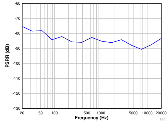
图 17. Power-Supply Rejection Ratio vs Ripple Frequency With 1- V_{PP} Amplitude
