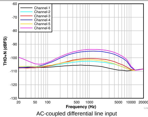
图 6. THD+N vs Input Frequency With a -1-dBr Input
