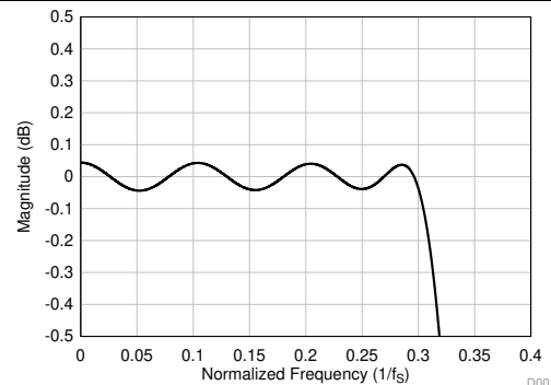
图 57. Linear Phase Decimation Filter Pass-Band Ripple
