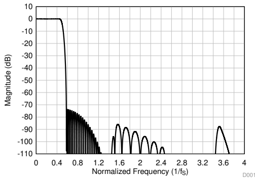
图 54. Linear Phase Decimation Filter Magnitude Response
