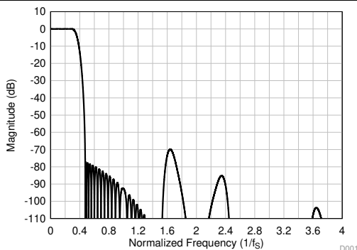
图 56. Linear Phase Decimation Filter Magnitude Response
