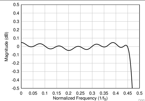
图 49. Linear Phase Decimation Filter Pass-Band Ripple
