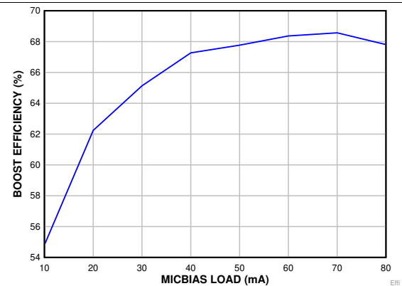
图 19. Boost Efficiency vs MICBIAS Load Current
