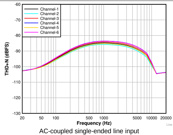
图 7. THD+N vs Input Frequency With a -1-dBr Input
