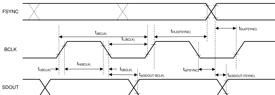
图 3. TDM/I²S/LJ Interface Timing Diagram
