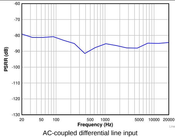
图 16. Power-Supply Rejection Ratio vs Ripple Frequency With 1- V_{PP} Amplitude
