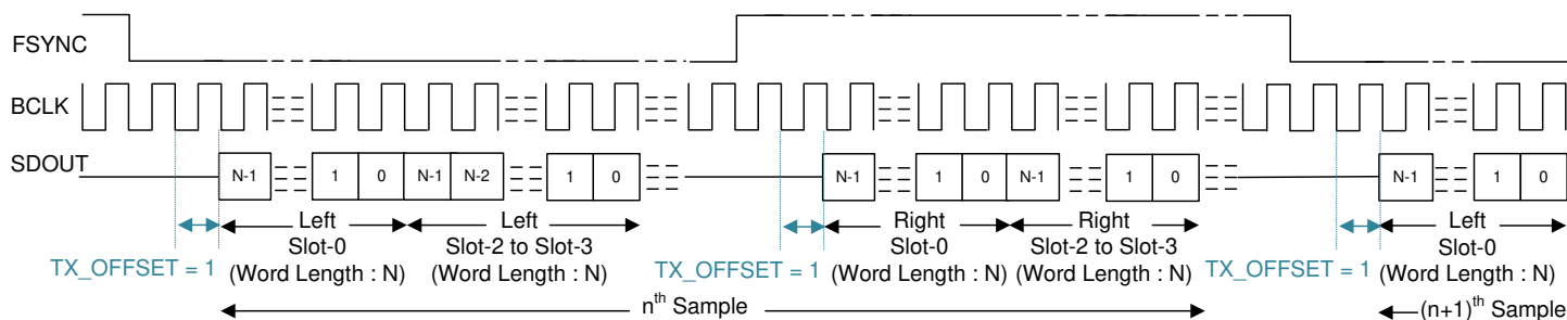
图 8-6. I²S Protocol Timing (TX_OFFSET = 1)
