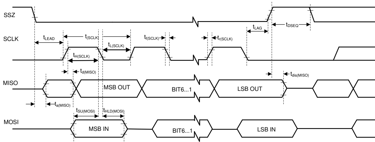
图 7-2. SPI Interface Timing Diagram
