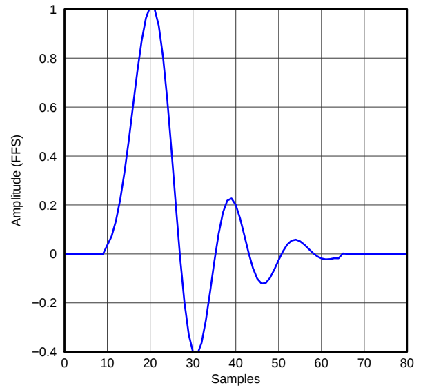
Figure 41. Asymmetric FIR x8 Interpolation Filter Impulse Response, Single Rate
