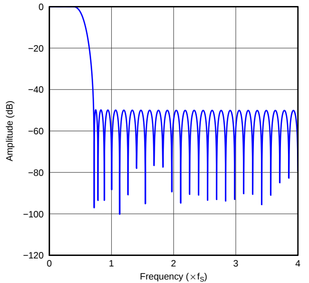
Figure 40. Asymmetric FIR x8 Interpolation Filter Frequency Response, Single Rate
