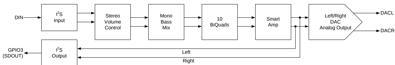
Figure 58. Example Processflow
