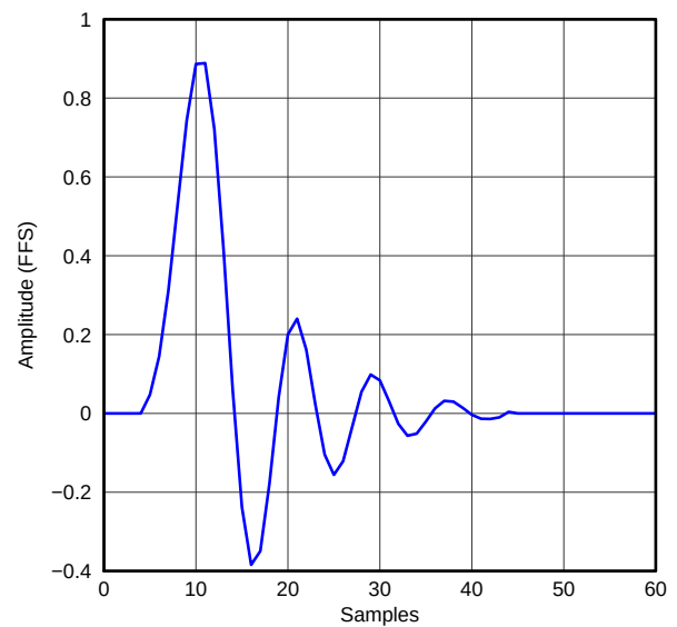
Figure 43. Asymmetric FIR x4 Interpolation Filter Impulse Response, Dual Rate
