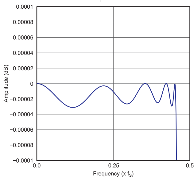
Figure 36. Low Latency x2 Interpolation Filter Passband Ripple
