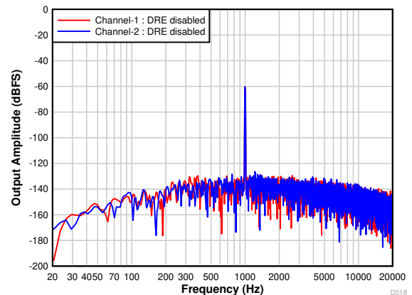
图 7-21. Differential FFT With a -60-dBr Input With DRE Disabled
