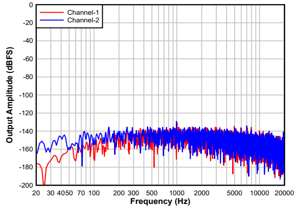
图 7-22. Single Ended FFT With Idle Input With DRE Enabled
