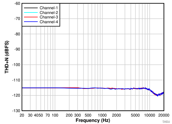
图 7-29. PDM Input THD+N vs Input Frequency With a -20-dBr Input
