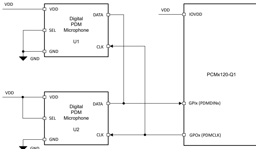
图 8-64. Digital PDM Microphones Connection Diagram for the PCM5120-Q1
