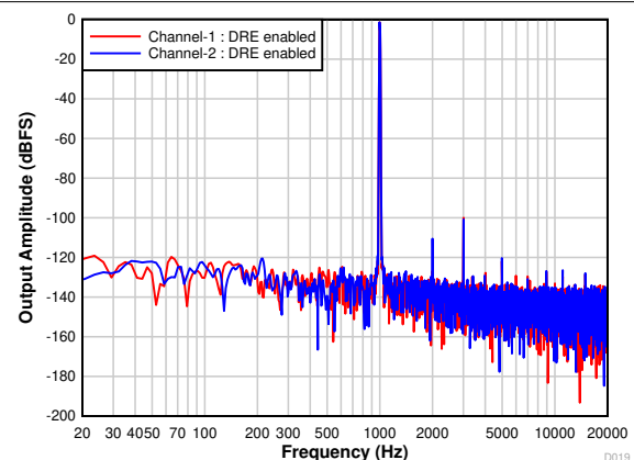
图 7-26. Differential FFT With a -1-dBr Input With DRE Enabled
