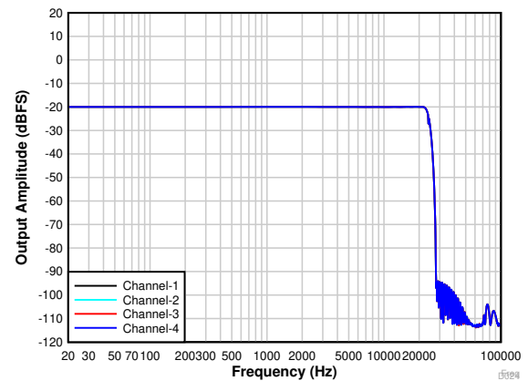
图 7-31. PDM Input Frequency Response With a -20-dBr Input
