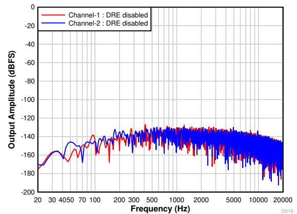
图 7-19. Differential FFT With Idle Input With DRE Disabled
