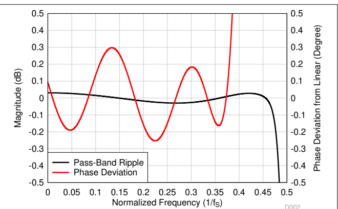
图 8-48. Low-Latency Decimation Filter Pass-Band Ripple and Phase Deviation
