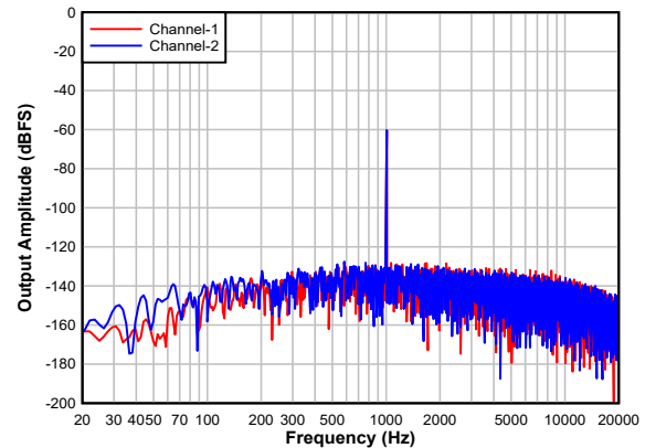
图 7-25. Single Ended FFT With a -60-dBr Input With DRE Disabled
