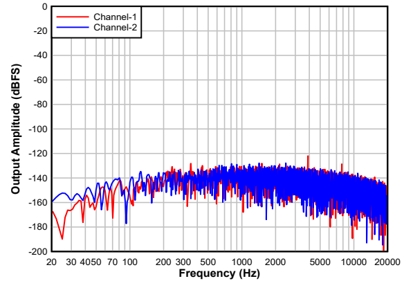
图 7-23. Single Ended FFT With Idle Input With DRE Disabled
