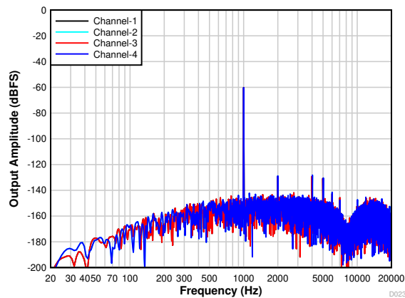
图 7-30. PDM Input FFT With a -60-dBr Input
