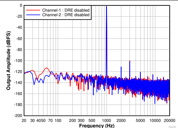
图 7-27. Differential FFT With a -1-dBr Input With DRE Disabled
