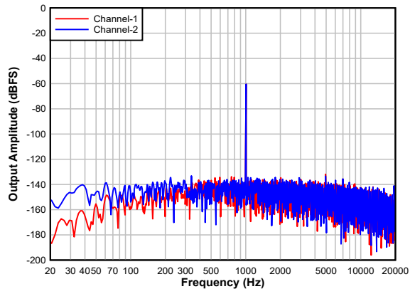
图 7-24. Single Ended FFT With a -60-dBr Input With DRE Enabled
