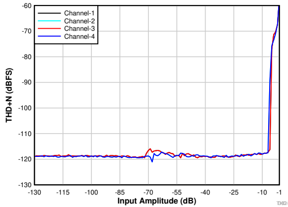
图 7-28. PDM Input THD+N vs Input Amplitude
