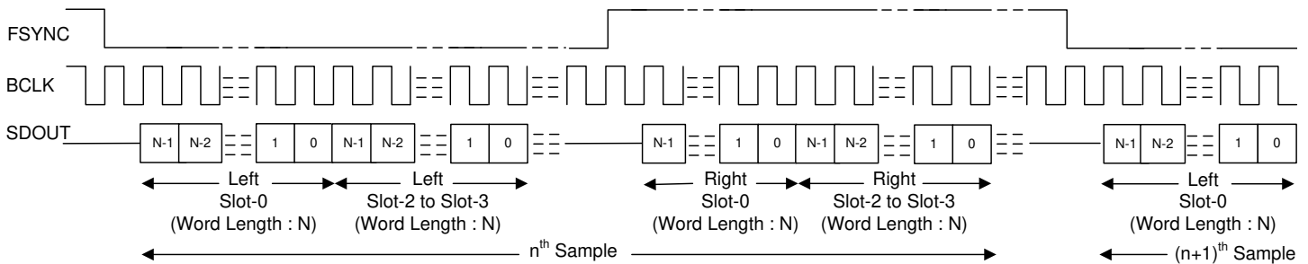
图 7-8. I²S 协议时序 (TX_OFFSET = 0 且 BCLK_POL = 1)
