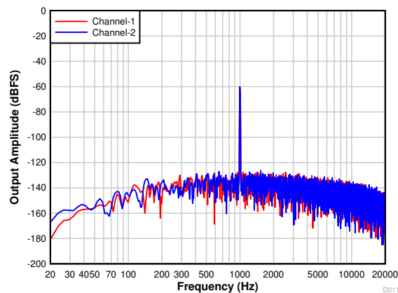
图 7-14. Differential FFT With a -60-dBr Input
