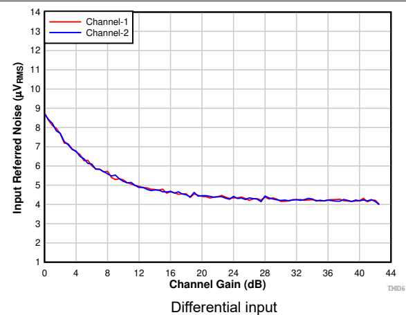
图 7-9. Input-Referred Noise vs Channel Gain
