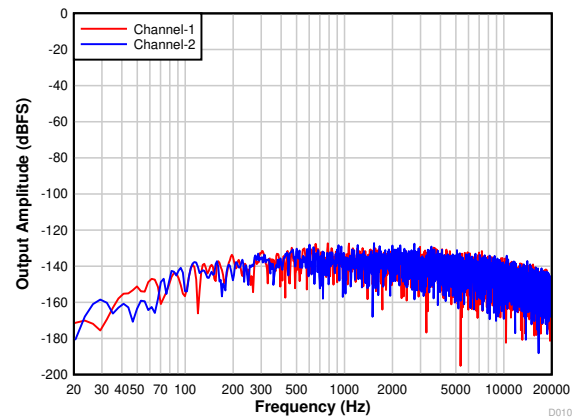
图 7-13. Differential FFT With Idle Input
