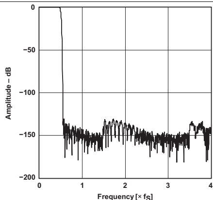
Figure 4. Amplitude vs Frequency Frequency Response, Sharp Rolloff
