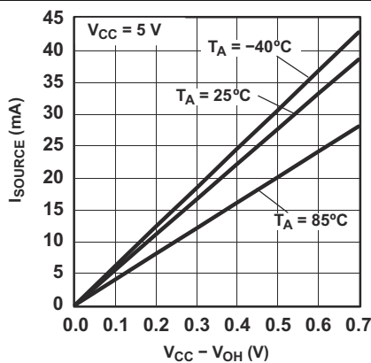
图 6-10. I/O Source Current vs Output High Voltage
