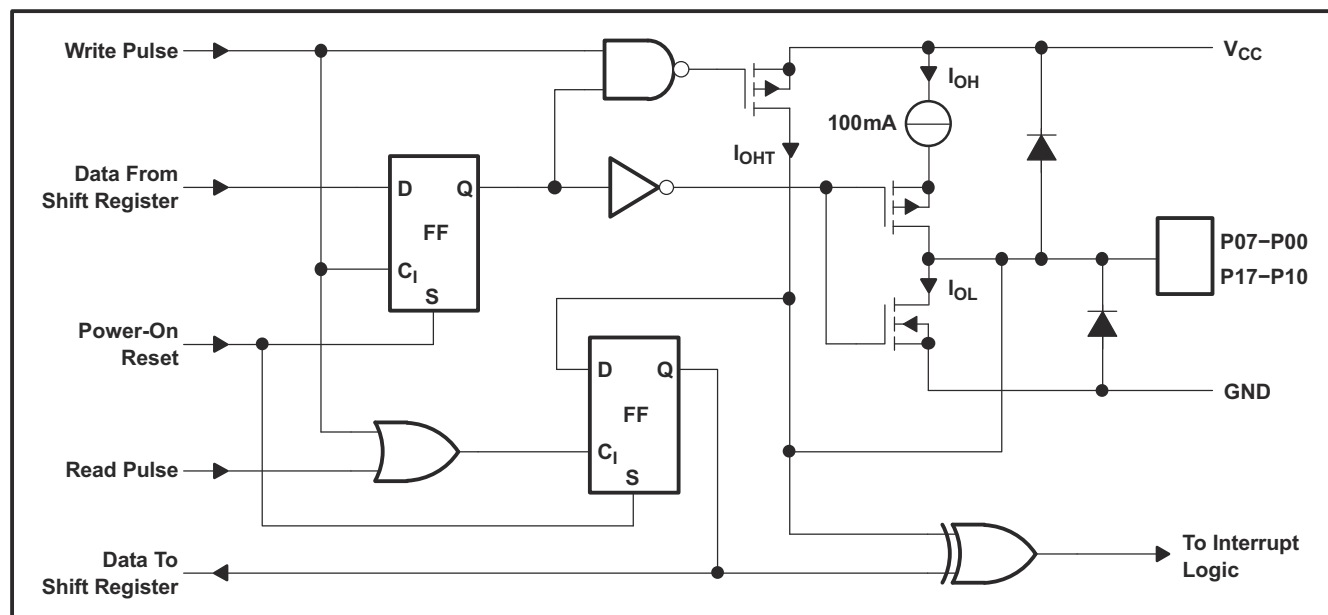
图 8-2. Simplified Schematic Diagram of Each P-Port Input or Output
