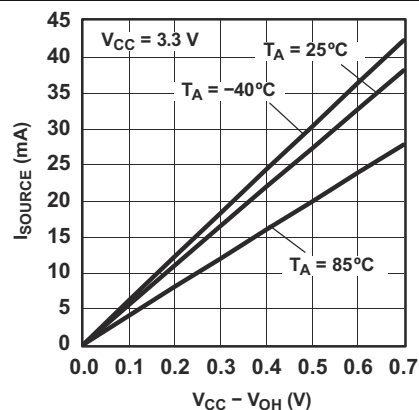
图 6-9. I/O Source Current vs Output High Voltage
