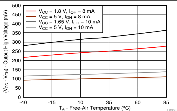
图 5-6. Output High Voltage ( V_{CC} - V_{OH} ) vs Temperature ( T_A ) for P-Ports
