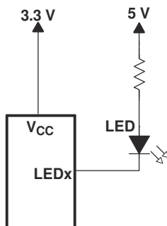
图 10-3. Device Supplied By A Lower Voltage
