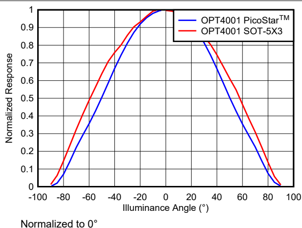
图 7-2. Device Response vs Illuminance Angle
