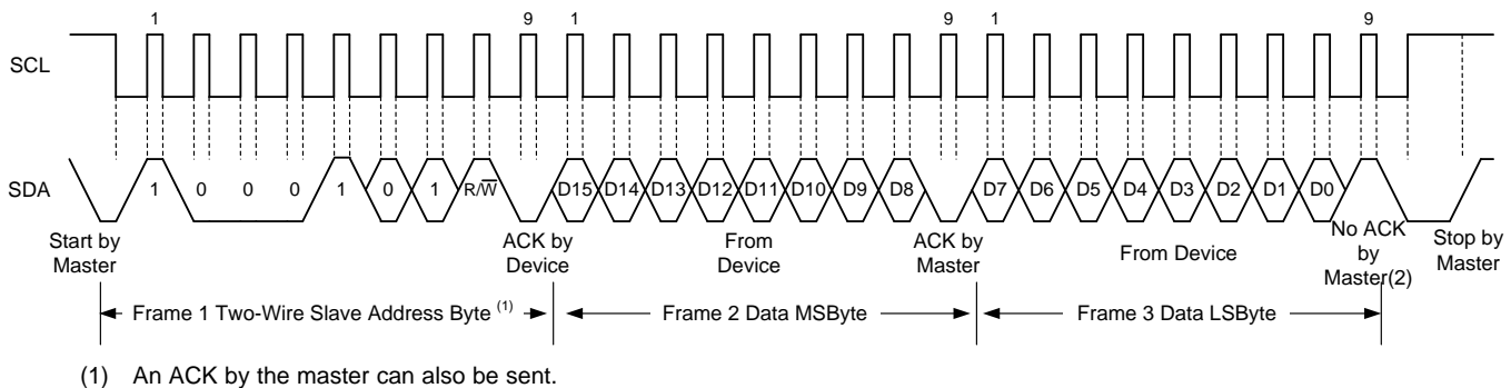
Figure 21. I²C Read Example
