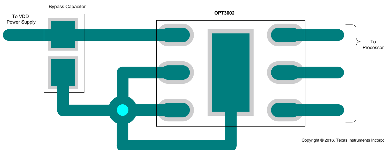
Figure 24. Example PCB Layout with the OPT3002
