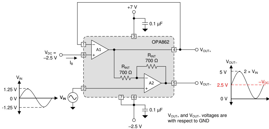
图 8-10. Level-Shifting With a DC Source of Polarity Opposite to the Desired DC Shift
