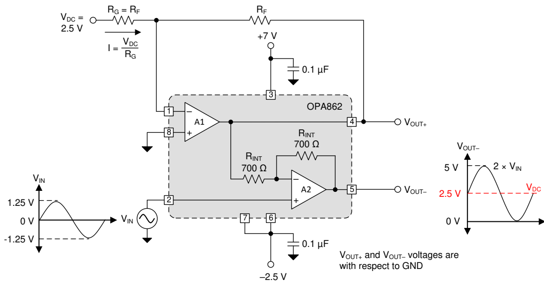
8-11. Level-Shifting With a DC Source of Polarity Same as the Desired DC Shift
