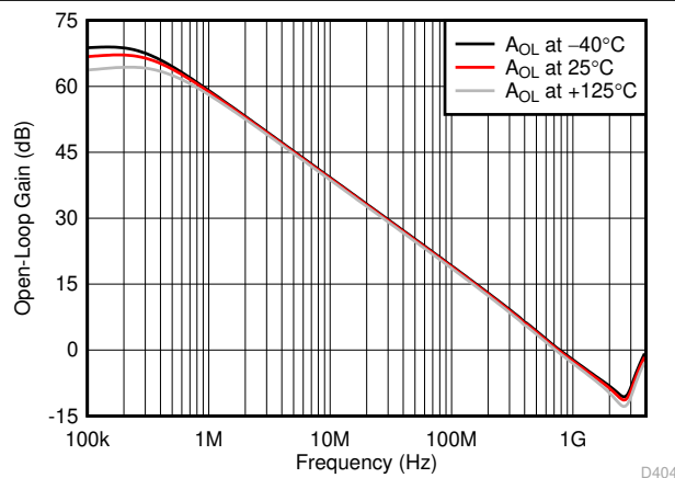
图 8-5. Open-Loop Gain vs Temperature
