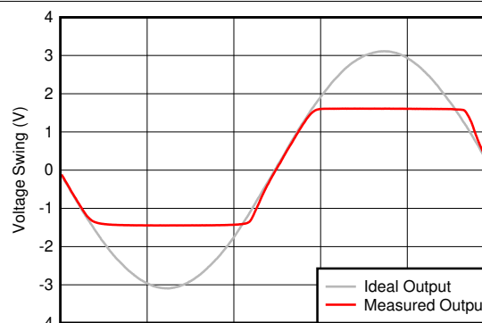
图 6-20. Large-Signal Transient Response
