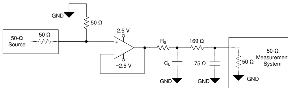
图 7-4. Capacitive Load Driver Configuration
