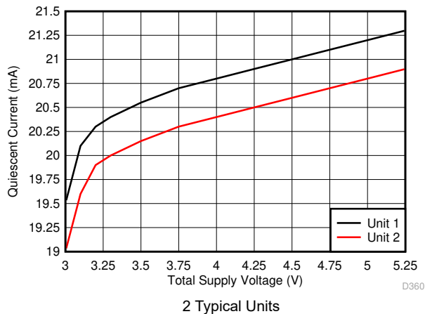
图 6-27. Quiescent Current vs Supply Voltage
