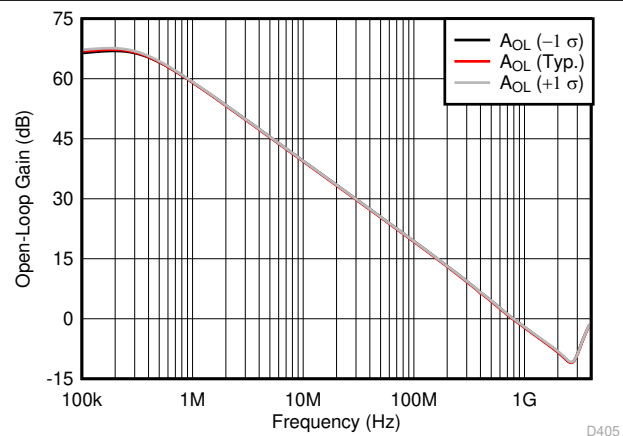
图 8-6. Open-Loop Gain vs Process Variation
