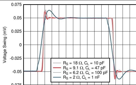
图 6-19. Small-Signal Transient Response
