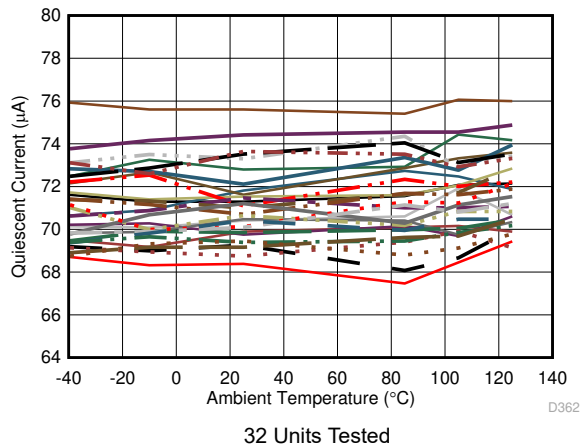
图 6-29. Quiescent Current (Amplifier Disabled) vs Ambient Temperature
