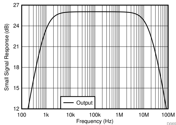
图 7-13. Inverting Single-Supply Response With AC-Coupled Input
