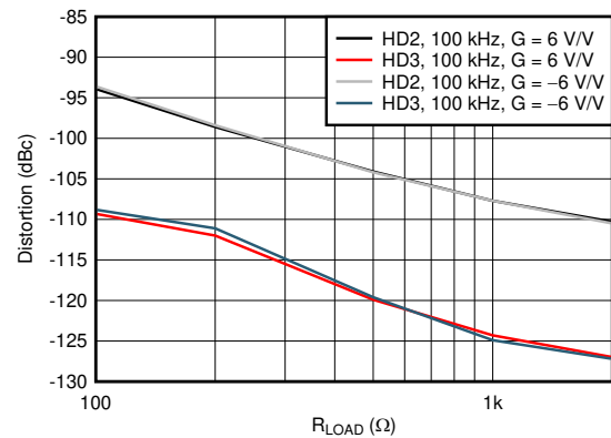
图 6-32. Harmonic Distortion vs Load
