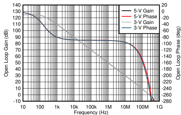
图 6-37. Open-Loop Gain and Phase
