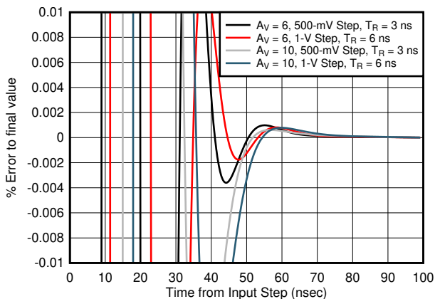
图 6-25. Noninverting Step Response vs V_{OPP}
