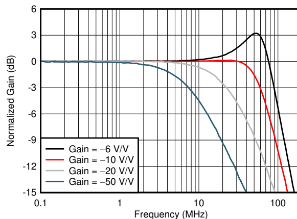
图 6-20. Inverting Small-Signal Response vs Gain
