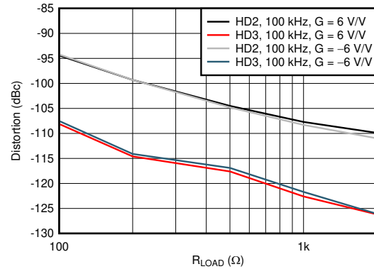
图 6-14. Harmonic Distortion vs R_{LOAD}
