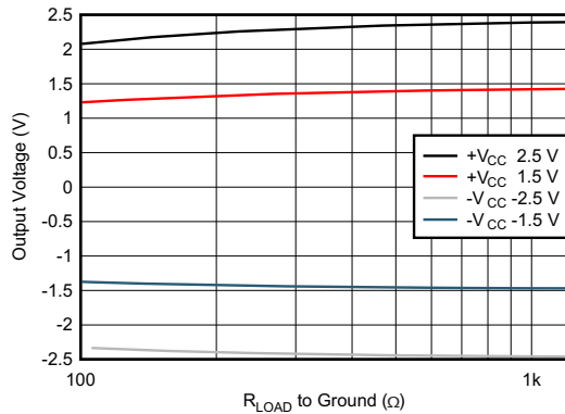
图 6-55. Output Voltage Swing vs Load Resistor
