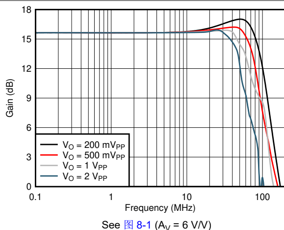
图 6-21. Noninverting Large-Signal Bandwidth vs V_{OPP}
