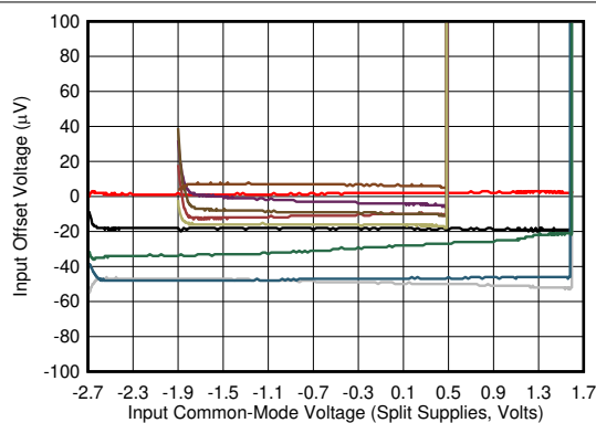
图 6-59. Input Offset Voltage vs Input Common-Mode Voltage
