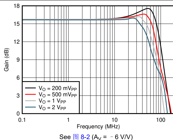
图 6-22. Inverting Large-Signal Bandwidth vs V_{OPP}
