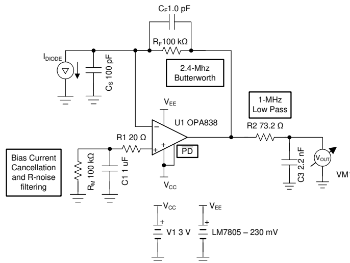
图 8-7. 100-kΩ Wide Bandwidth Transimpedance Design
