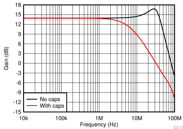
图 7-5. Inverting Response With and Without Compensation
