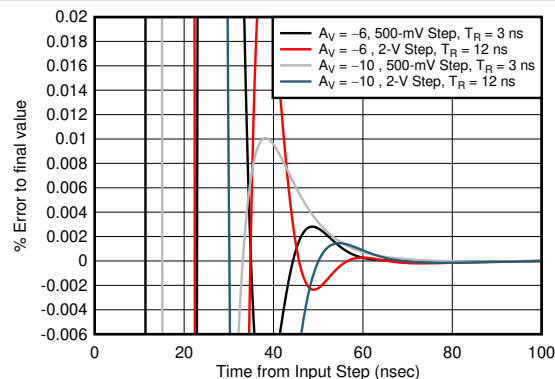
图 6-8. Inverting Step Response vs V_{OPP}
