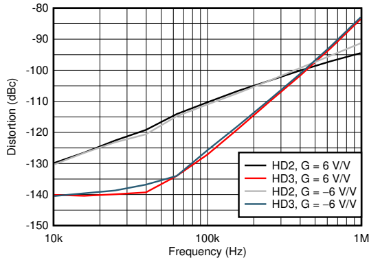
图 6-13. Harmonic Distortion vs Frequency
