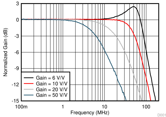
图 6-1. Noninverting Small-Signal Frequency Response vs Gain
