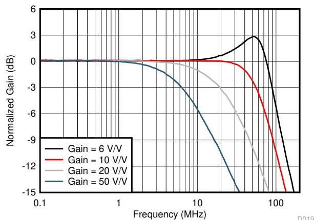
图 6-19. Noninverting Small-Signal Response vs Gain
