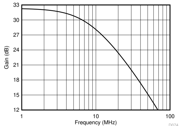
图 8-6. Differential Small-Signal Frequency Response
