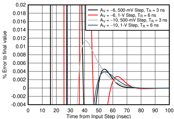
图 6-26. Inverting Step Response vs V_{OPP}
