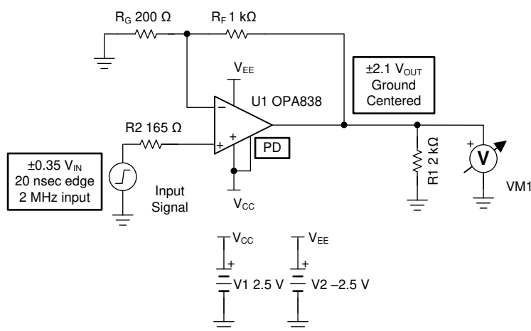
图 7-8. Split-Supply Operation
