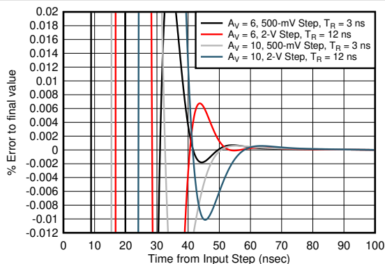
图 6-7. Noninverting Step Response vs V_{OPP}
