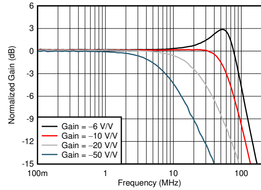
图 6-2. Inverting Small-Signal Frequency Response vs Gain
