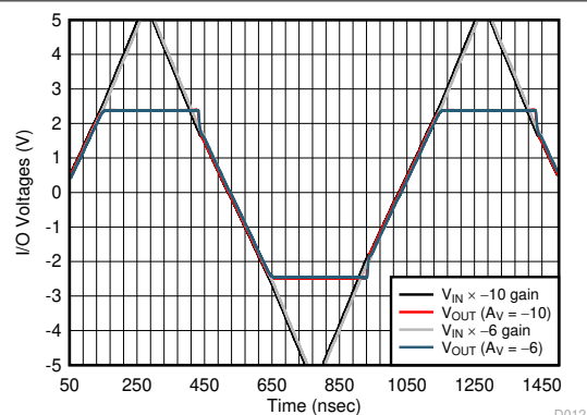
图 6-10. Simulated Inverting Settling Time
