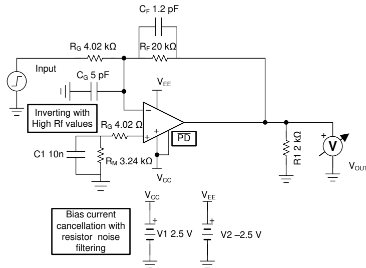
图 7-4. G = -5 V/V With Optional Compensation
