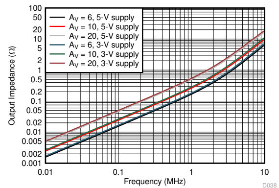
图 6-38. Closed-Loop Output Impedance
