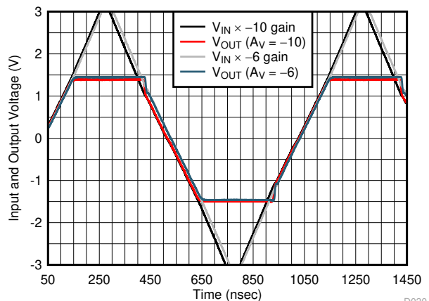
图 6-28. Inverting Settling Time
