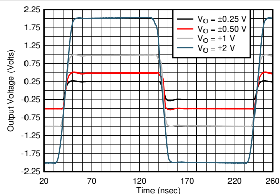
图 6-8. Inverting Step Response vs V_{OPP}
