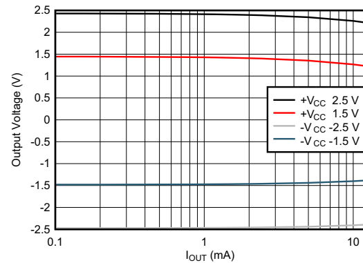
图 6-56. Output Saturation Voltage vs Load Current
