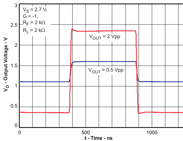
图 7-4. Inverting Pulse Response
