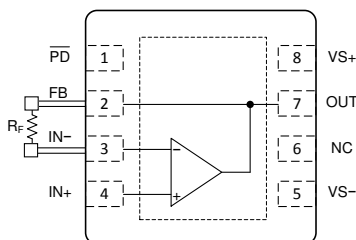
图 7-4. R_F Connection Between FB and IN - Pins
