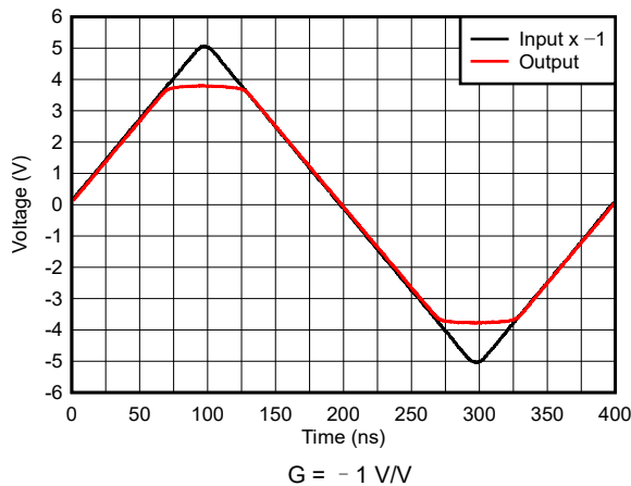
图 6-33. Inverting Output Overdrive Recovery
