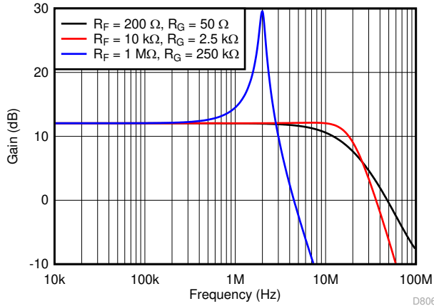
图 8-8. Closed-Loop Gain vs. Frequency for Circuit of 图 8-5
