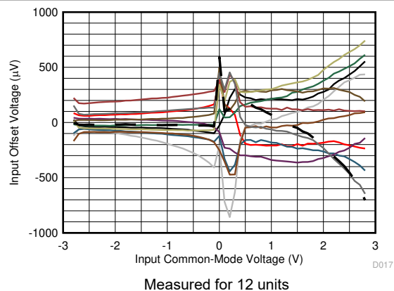
图 6-41. Input Offset Voltage vs Input Common-Mode Voltage
