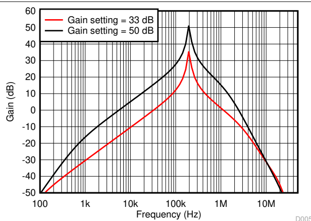
图 9-11. Hi-Z, High-Gain Front-End Circuit Gain vs Frequency
