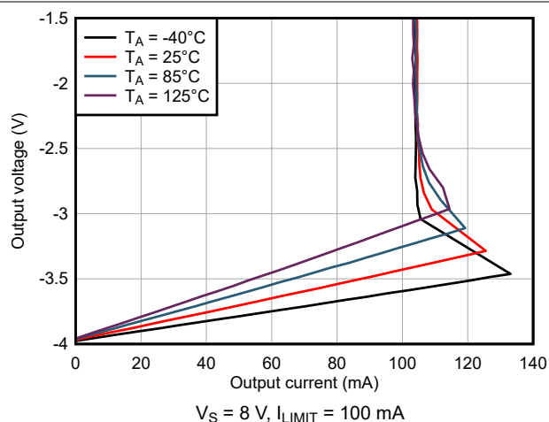
图 6-20. Output Voltage vs Output Sinking Current
