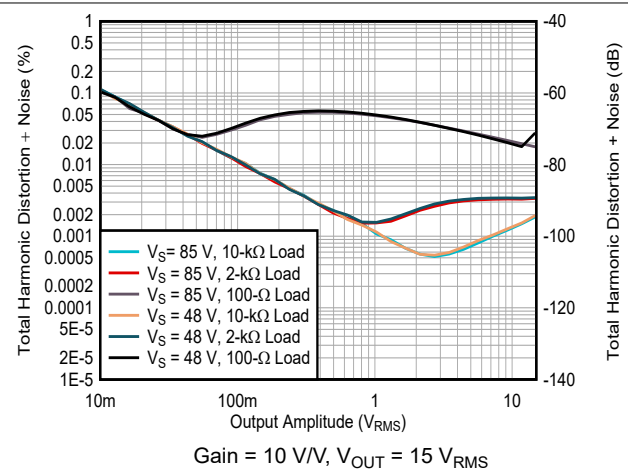
图 6-48. Total Harmonic Distortion + Noise vs Amplitude
