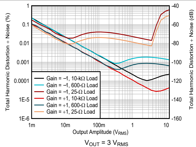
图 6-46. Total Harmonic Distortion + Noise vs Amplitude
