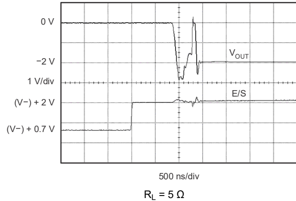
Figure 5-16. Enable Response
