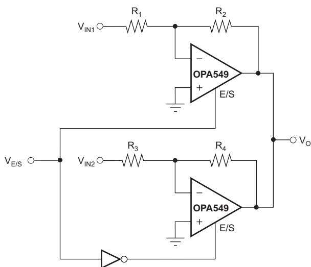
Figure 14. Switched Amplifier
