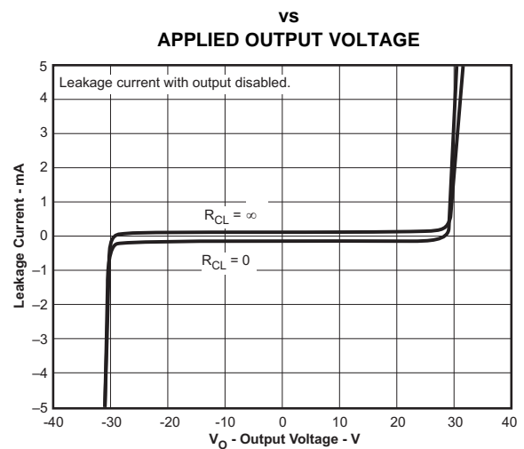
OUTPUT LEAKAGE CURRENT
