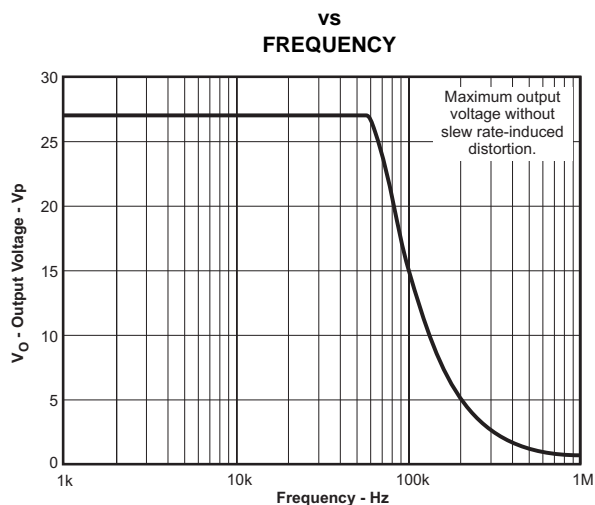
MAXIMUM OUTPUT VOLTAGE SWING
