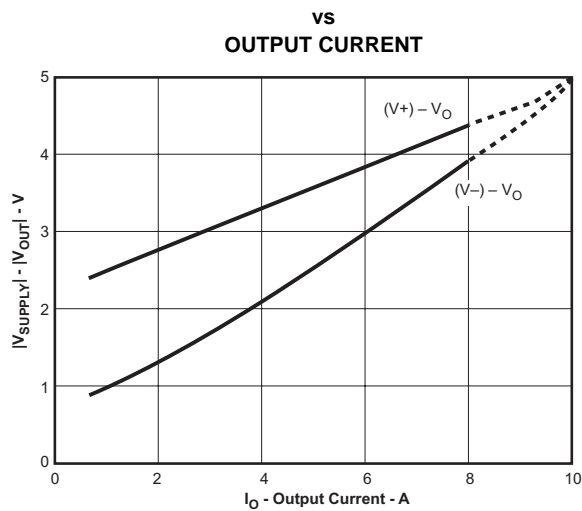
MAXIMUM OUTPUT VOLTAGE SWING
