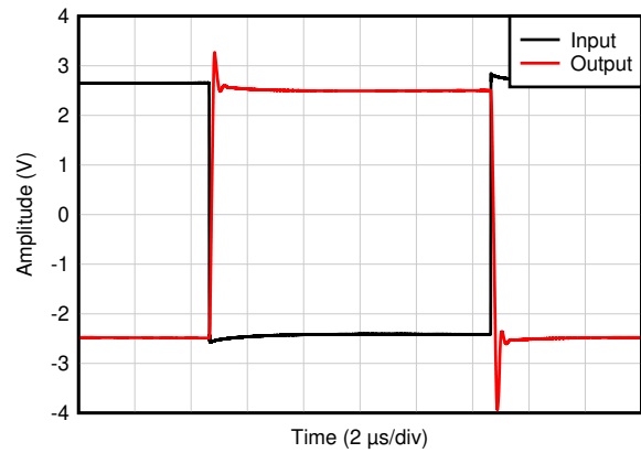
图 5-40. Large-Signal Step Response
