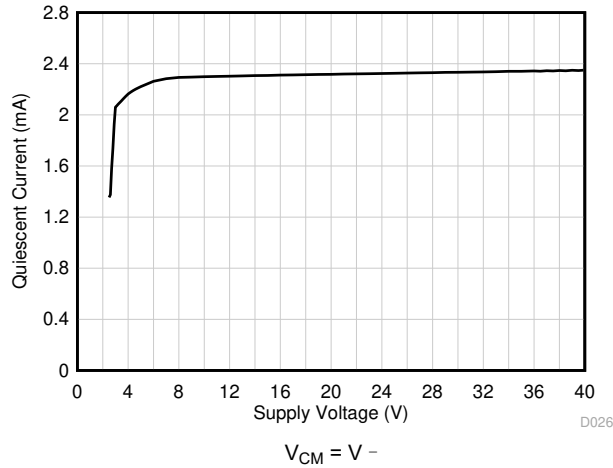
图 5-27. Quiescent Current vs Supply Voltage
