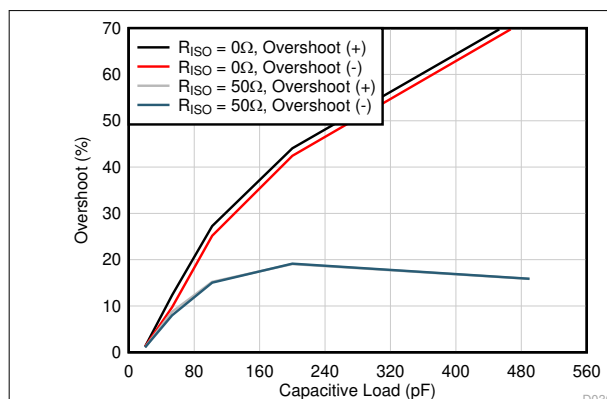
图 6-5. Small-Signal Overshoot vs Capacitive Load (20mV pp Output Step, G = +1)
