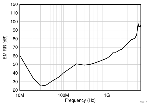
图 5-43. EMIRR (Electromagnetic Interference Rejection Ratio) vs Frequency
