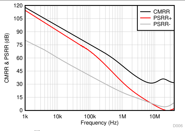
图 5-20. CMRR and PSRR vs Frequency
