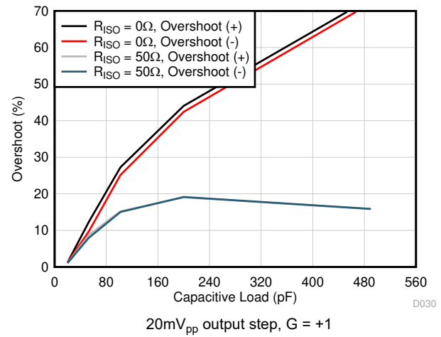
图 5-32. Small-Signal Overshoot vs Capacitive Load
