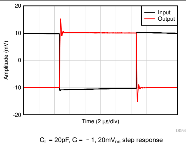
图 5-38. Small-Signal Step Response
