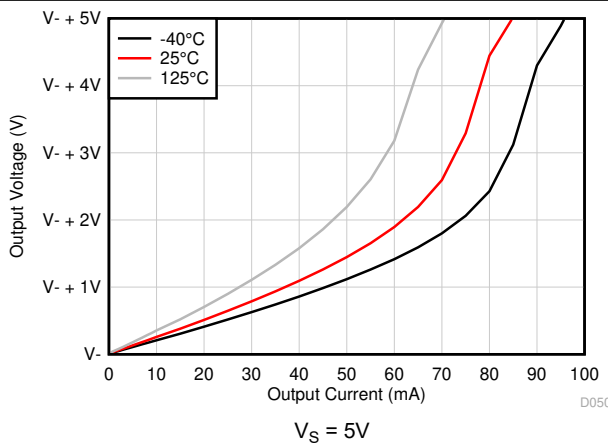
图 5-19. Output Voltage Swing vs Output Current (Sinking)
