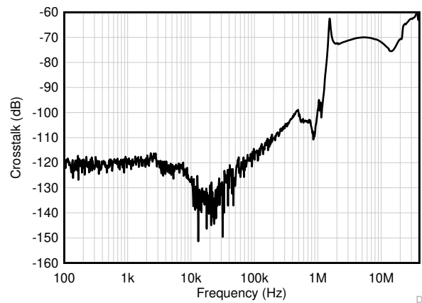
图 5-42. Channel Separation vs Frequency
