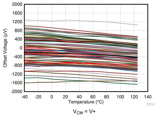
V_{CM} = V^+ Data from 74 amplifiers 图 5-4. Offset Voltage vs Temperature
