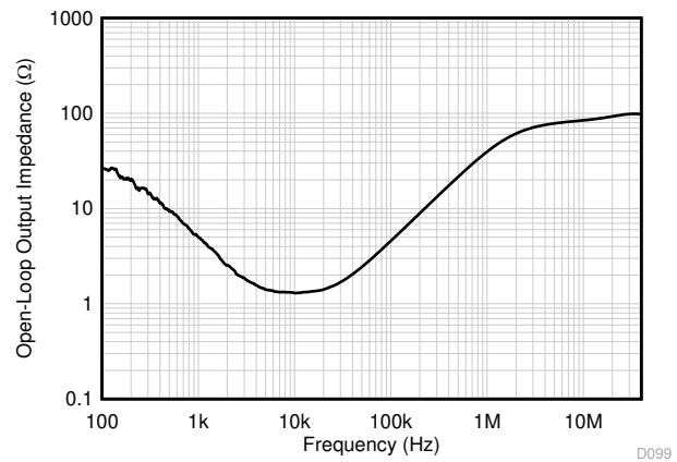
图 5-30. Open-Loop Output Impedance vs Frequency
