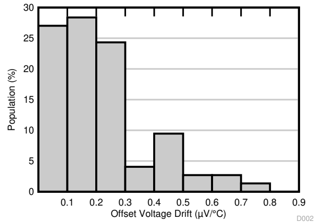
Distribution from 74 amplifiers 图 5-2. Offset Voltage Drift Distribution
