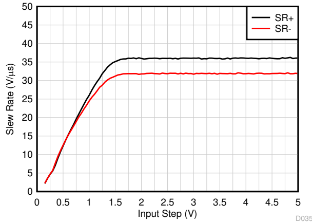
图 5-15. Slew Rate vs Input Step Voltage
