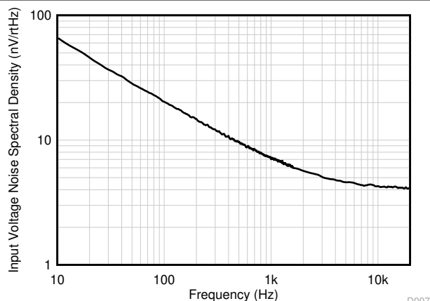
图 5-26. Input Voltage Noise Spectral Density vs Frequency
