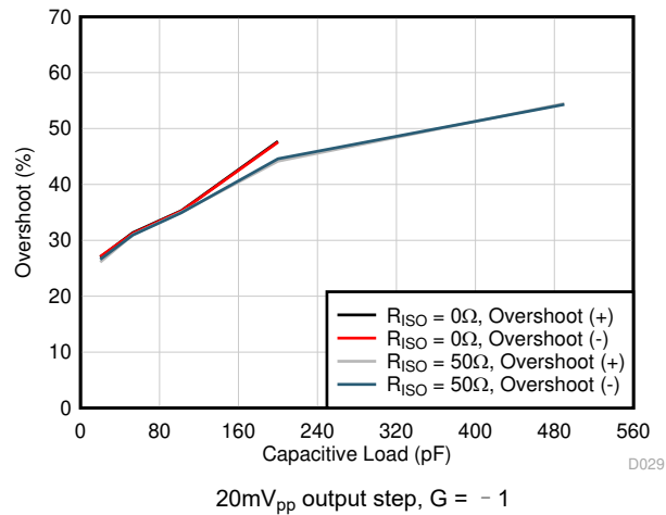
图 5-31. Small-Signal Overshoot vs Capacitive Load
