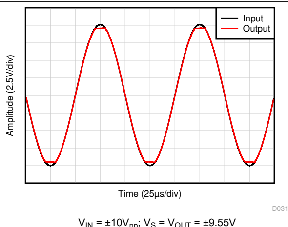
图 5-34. No Phase Reversal
