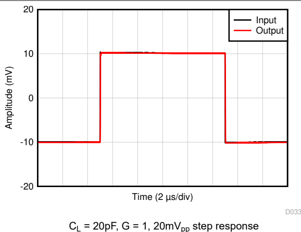
图 5-37. Small-Signal Step Response
