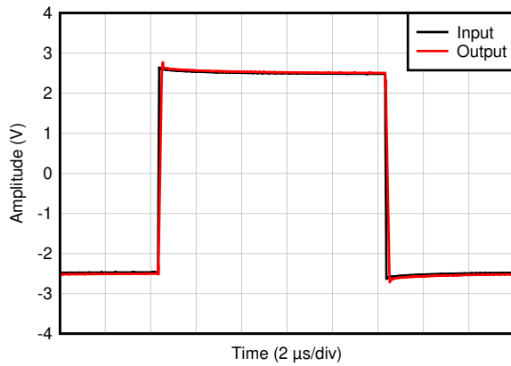
图 5-39. Large-Signal Step Response
