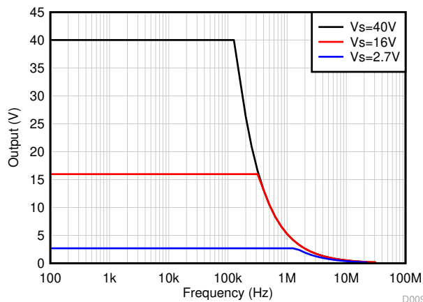
图 5-41. Maximum Output Voltage vs Frequency
