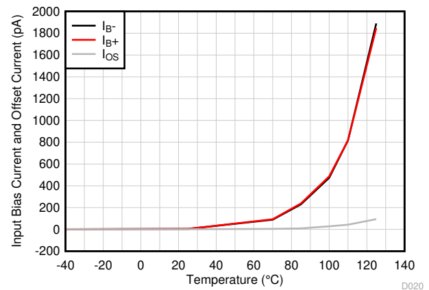
图 5-14. Input Bias Current and Offset Current vs Temperature
