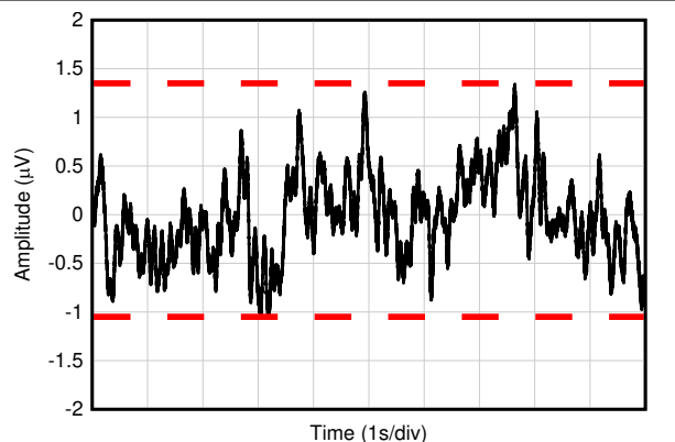
图 5-25. 0.1Hz to 10Hz Noise
