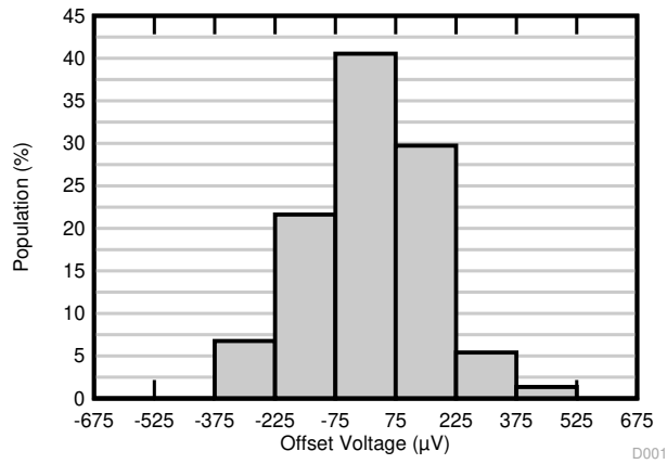
Distribution from 74 amplifiers, T_A = 25^\circ\text{C} 图 5-1. Offset Voltage Production Distribution
