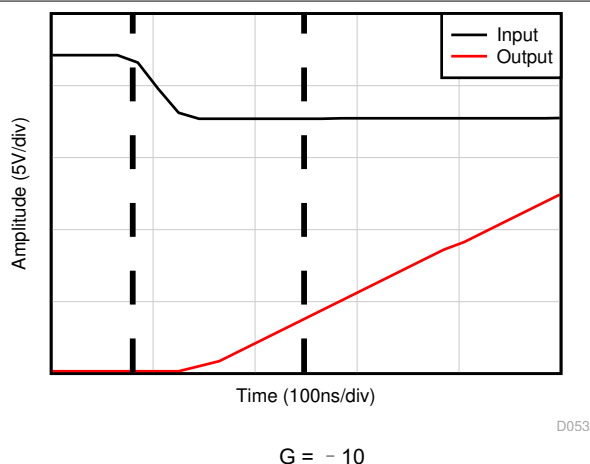
图 5-36. Negative Overload Recovery
