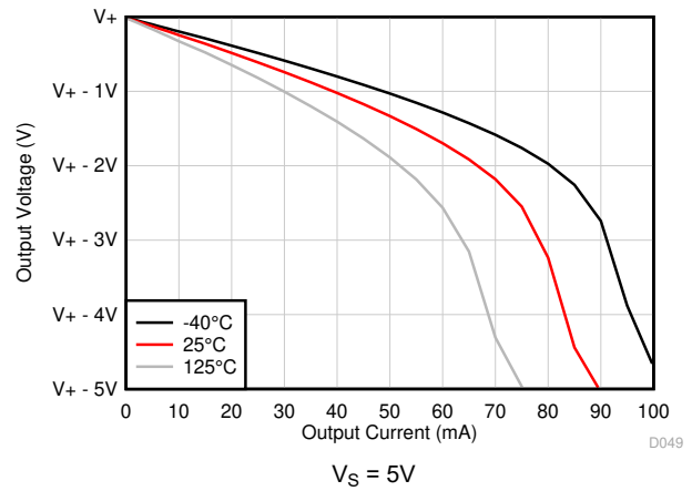
图 5-18. Output Voltage Swing vs Output Current (Sourcing)
