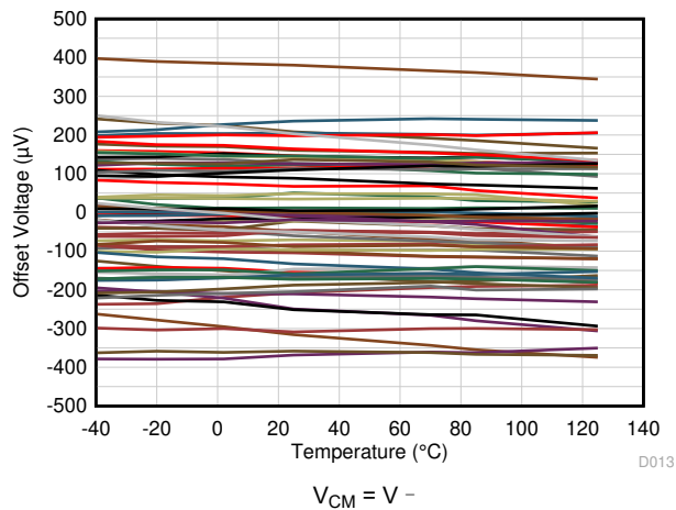
V_{CM} = V^- Data from 74 amplifiers 图 5-3. Offset Voltage vs Temperature
