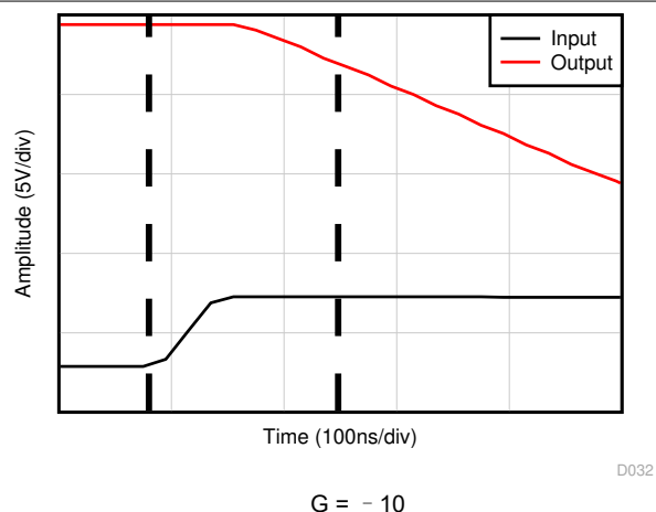
图 5-35. Positive Overload Recovery
