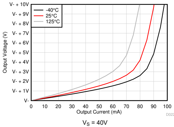
图 5-17. Output Voltage Swing vs Output Current (Sinking)
