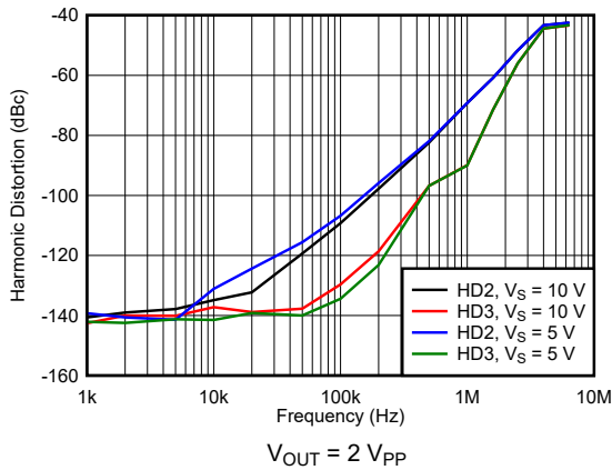
图 7-51. Harmonic Distortion vs Supply Voltage
