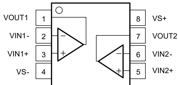
图 6-3. OPA2863 D Package, 8-Pin SOIC and DGK Package, 8-Pin VSSOP, (Top View)
