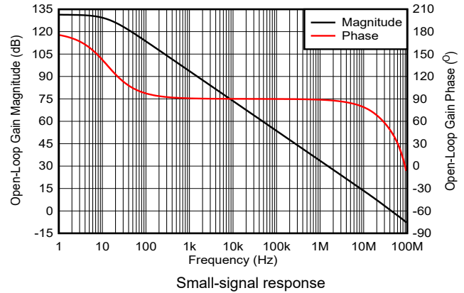
图 7-50. Open-Loop Gain and Phase vs Frequency
