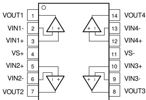
图 6-5. OPA4863 PW Package, 14-Pin TSSOP (Top View)
