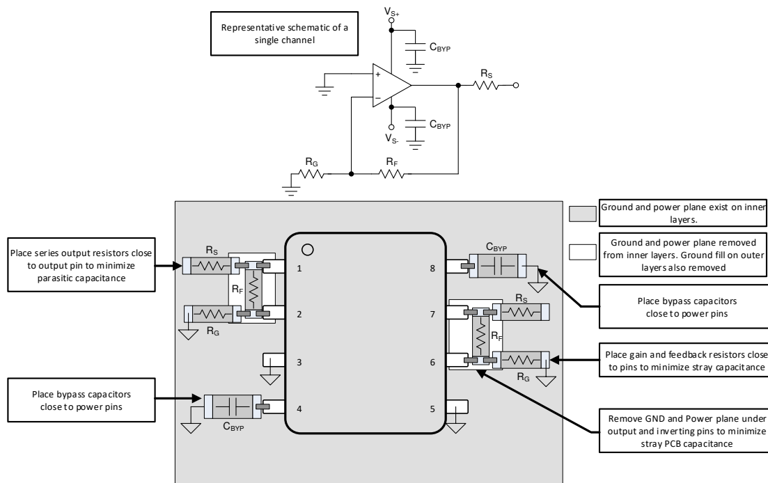
图 9-7. Layout Recommendation for Dual-Channel DGK Package
