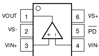
图 6-1. OPA863 DBV Package, 6-Pin SOT-23 (Top View)
