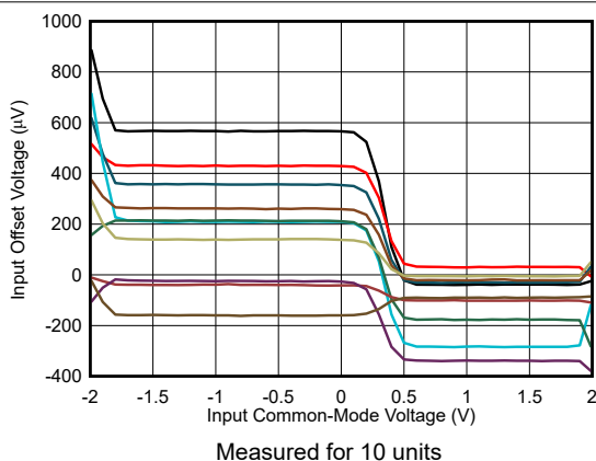
图 7-35. Input Offset Voltage vs Input Common-Mode Voltage
