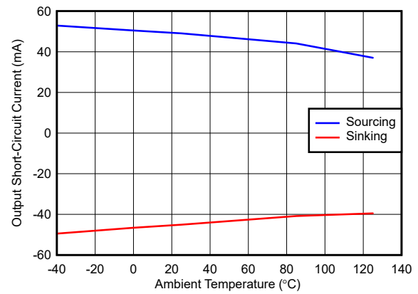
图 7-38. Output Short-Circuit Current vs Ambient Temperature
