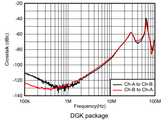
图 7-52. Crosstalk vs Frequency
