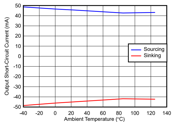
Output saturated and then short-circuited to opposite supply 图 7-18. Output Short-Circuit Current vs Ambient Temperature
