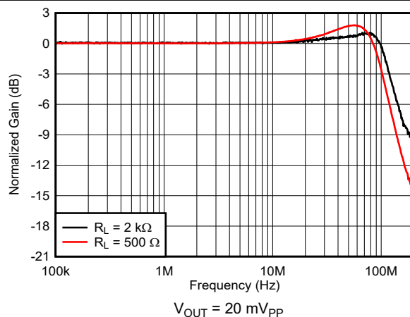
图 7-2. Small-Signal Frequency Response vs Output Load
