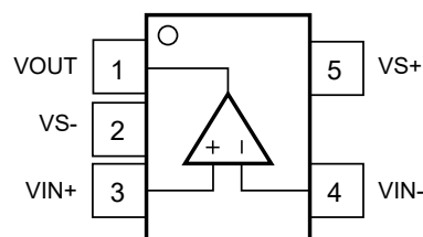
图 6-2. OPA863 DBV Package, 5-Pin SOT-23 (Top View)
