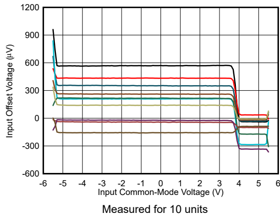
图 7-15. Input Offset Voltage vs Input Common-Mode Voltage
