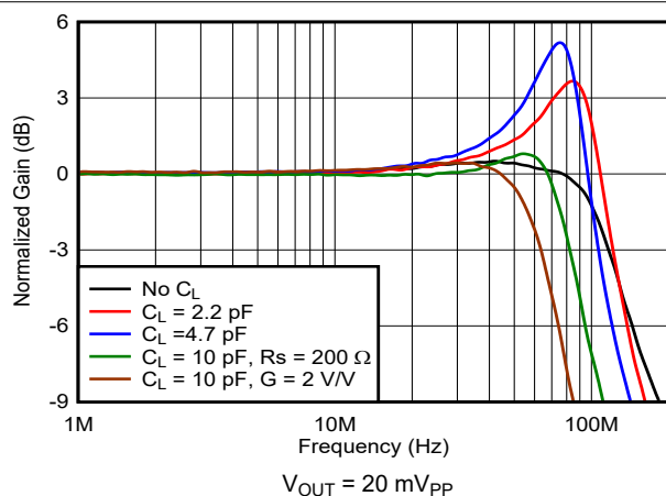
图 7-3. Frequency Response vs Load Capacitance
