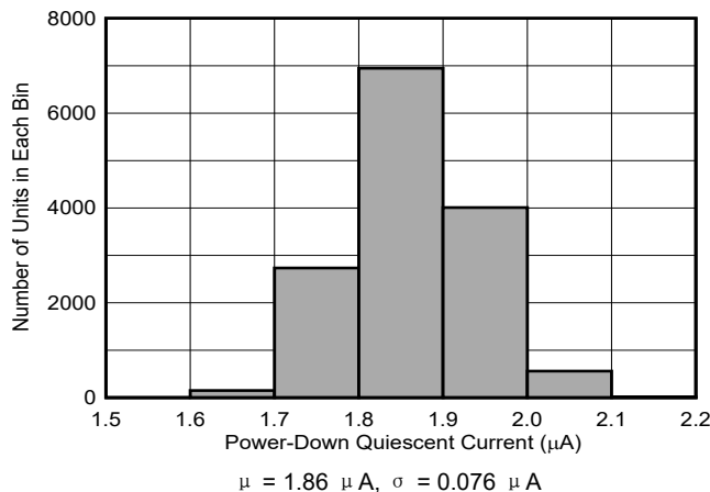
图 7-29. Power-Down Quiescent Current Distribution
