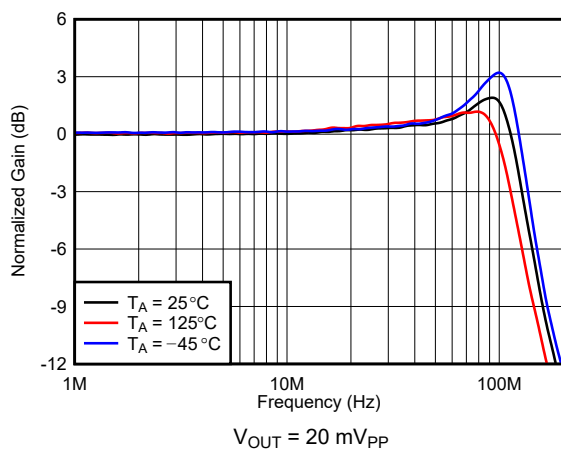
图 7-5. Frequency Response vs Ambient Temperature
