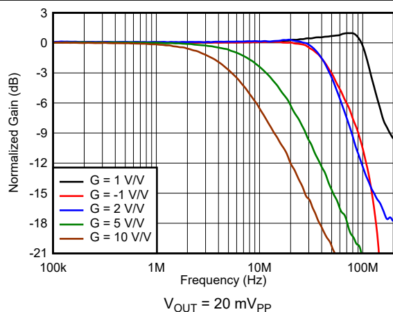
图 7-1. Small-Signal Frequency Response vs Gain
