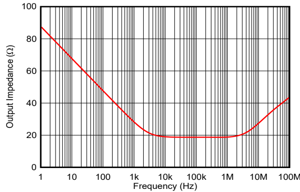
图 7-49. Open-Loop Output Impedance vs Frequency
