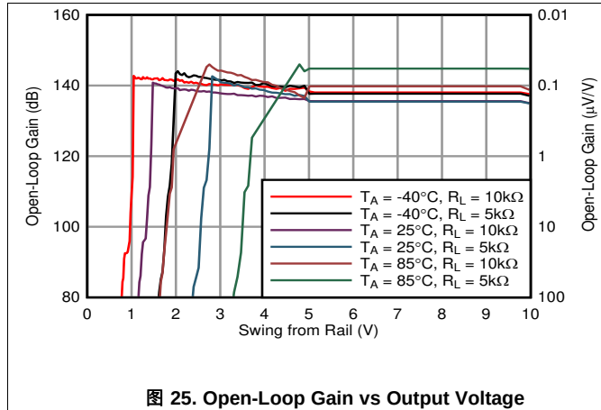
图 25. Open-Loop Gain vs Output Voltage
