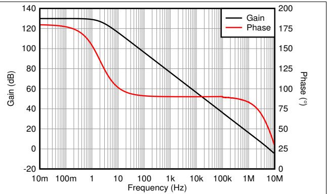
图 26. Open-Loop Gain and Phase vs Frequency
