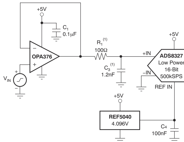
图 8-3. Driving an ADS8327
