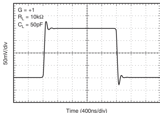
图 6-19. Small-Signal Pulse Response
