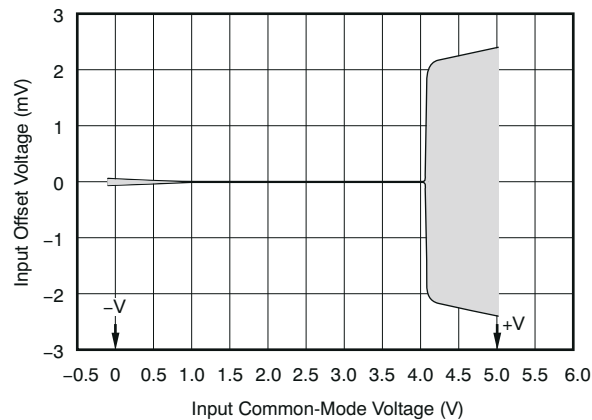
图 7-2. Offset and Common-Mode Voltage
