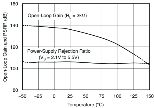
图 6-3. Open-Loop Gain and Power-Supply Rejection Ratio vs Temperature
