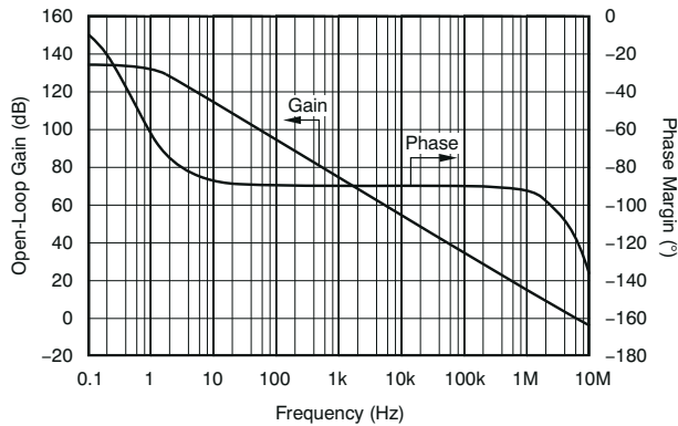
图 6-1. Open-Loop Gain and Phase vs Frequency
