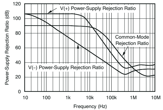
图 6-2. Power-Supply and Common-Mode Rejection Ratio vs Frequency
