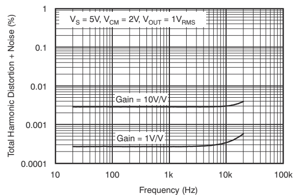
图 6-6. Total Harmonic Distortion + Noise vs Frequency
