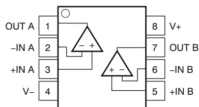
图 5-4. OPA2376-Q1: D (8-Pin SOIC) and DGK (8-Pin VSSOP) Packages, Top View
