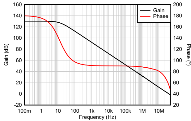
图 5-8. Open-Loop Gain/Phase vs Frequency
