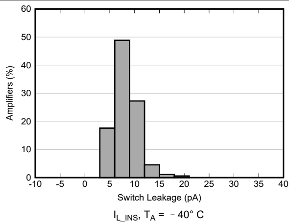
图 5-37. Switch Input Leakage Current Histogram
