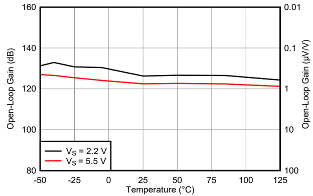
图 5-9. Open-Loop Gain vs Temperature
