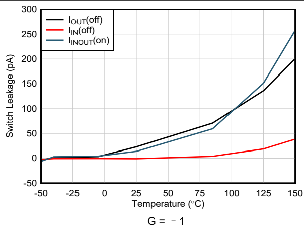
图 5-36. Switch Leakage Current vs Temperature
