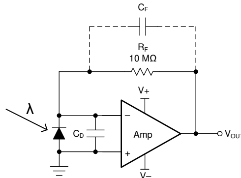
图 8-3. Dual-Supply Transimpedance Amplifier
