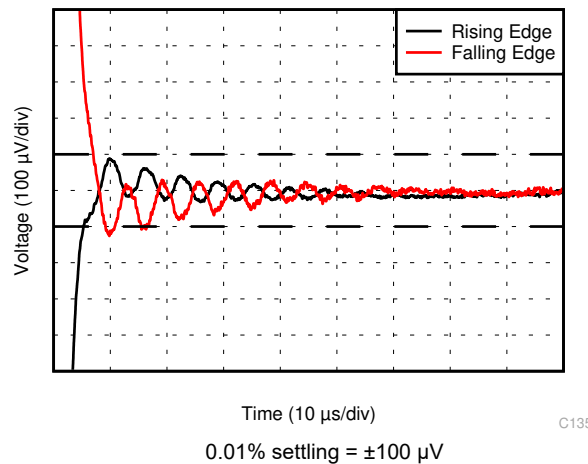
图 6-29. Settling Time
