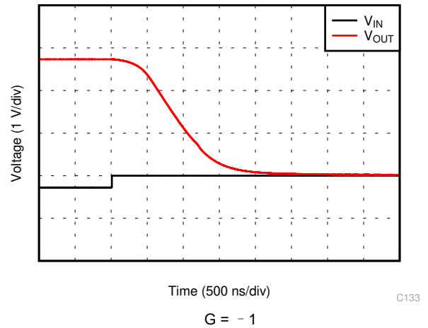
图 6-26. Overload Recovery
