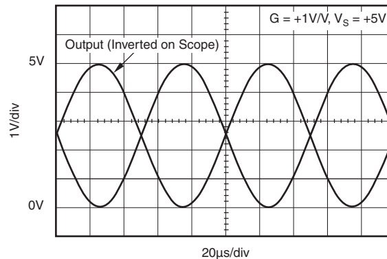
Figure 23. 轨至轨 I/O
