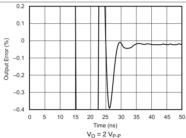
图 27. Output Settling Time to 0.1%
