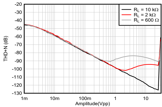
图 5-30. THD+N 与输出幅度间的关系 f = 1\text{ kHz} BW = 80\text{ kHz} G = +1
