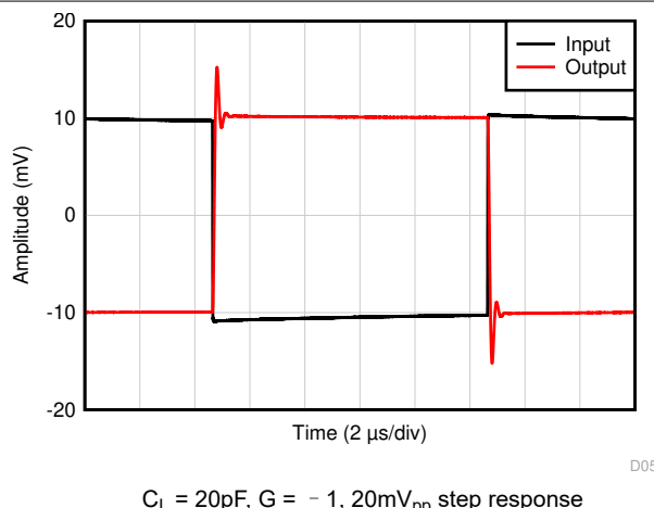
图 5-38. Small-Signal Step Response
