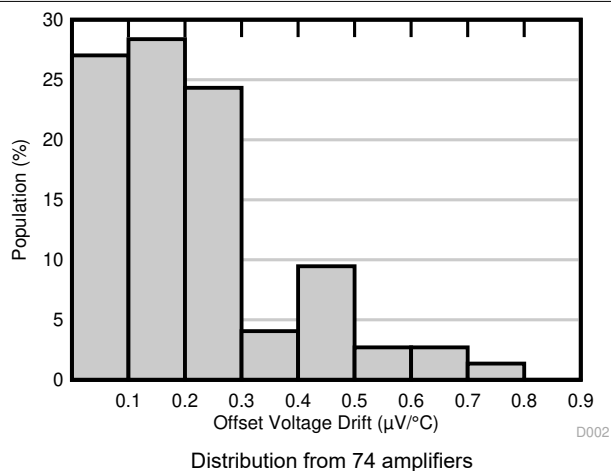
图 5-2. Offset Voltage Drift Distribution
