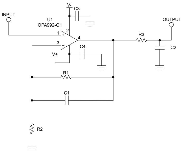
图 7-3. Schematic for Noninverting Configuration Layout Example
