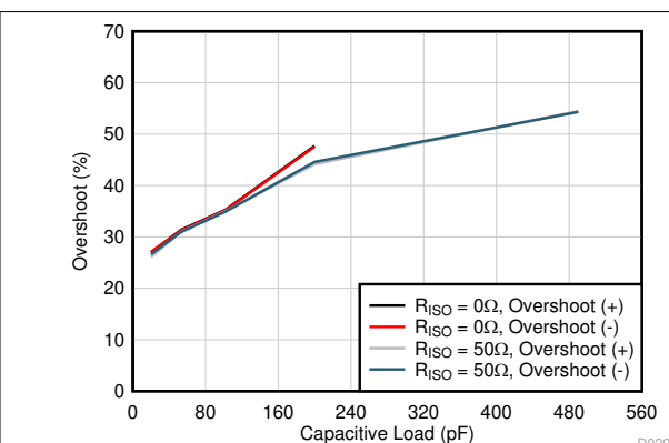
图 6-6. Small-Signal Overshoot vs Capacitive Load (20mV pp Output Step, G = -1)
