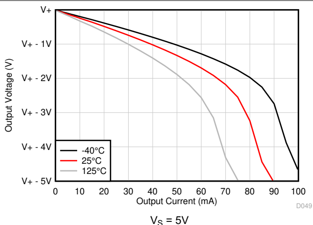
图 5-18. Output Voltage Swing vs Output Current (Sourcing)
