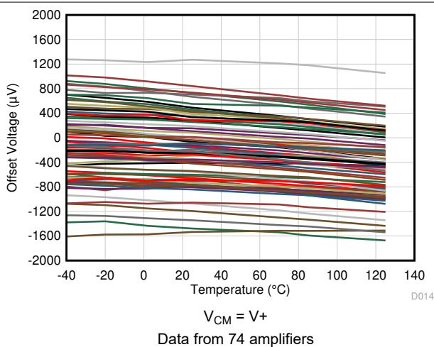
图 5-4. Offset Voltage vs Temperature
