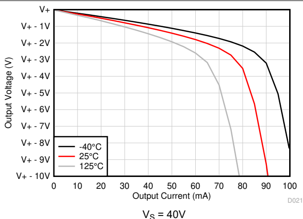
图 5-16. Output Voltage Swing vs Output Current (Sourcing)
