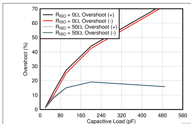
图 6-5. Small-Signal Overshoot vs Capacitive Load (20mV pp Output Step, G = +1)
