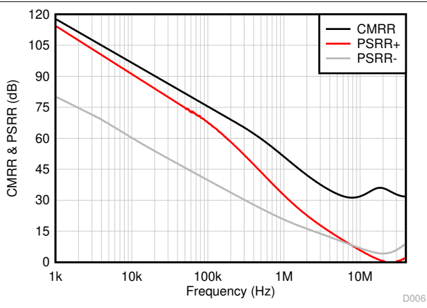
图 5-20. CMRR and PSRR vs Frequency
