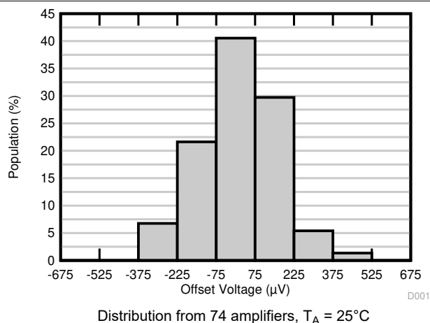
图 5-1. Offset Voltage Production Distribution
