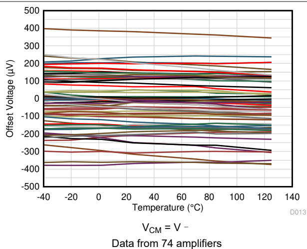
图 5-3. Offset Voltage vs Temperature
