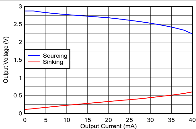
图 7-32. Output Voltage vs Load Current
