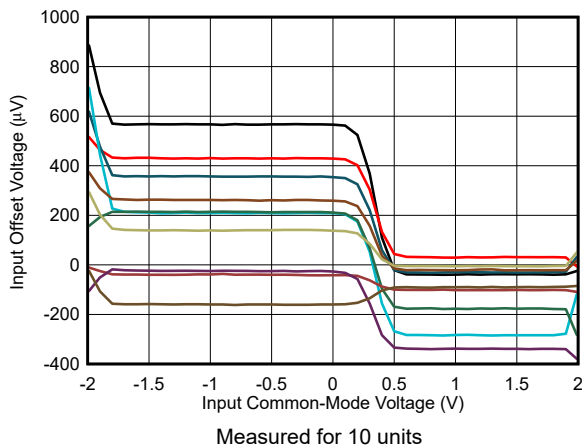
图 7-30. Input Offset Voltage vs Input Common-Mode Voltage
