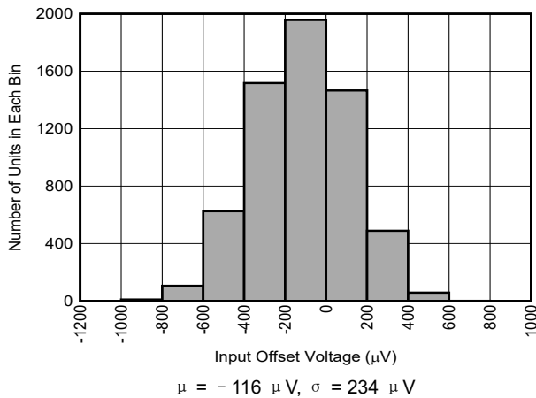
图 7-21. Input Offset Voltage Distribution
