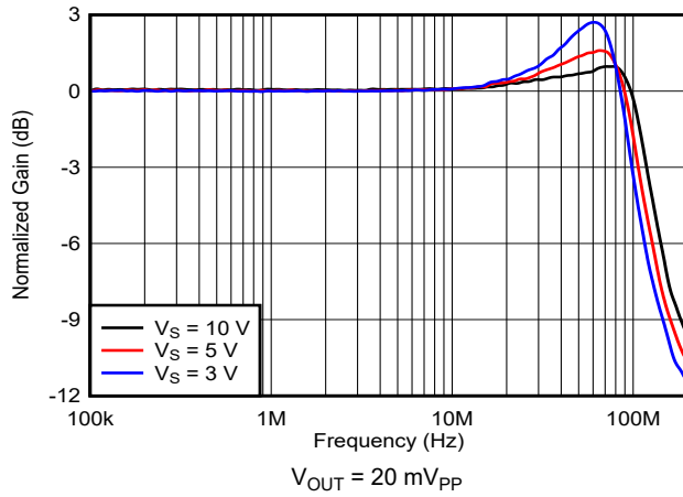
图 7-34. Frequency Response vs Supply Voltage
