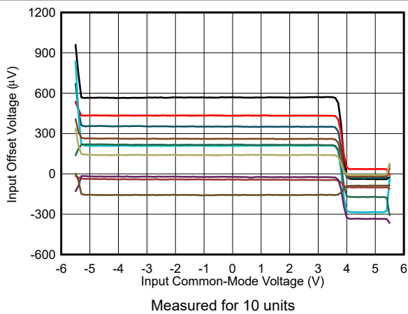
图 7-15. Input Offset Voltage vs Input Common-Mode Voltage
