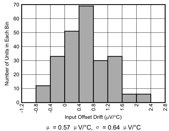
图 7-22. Input Offset Voltage Drift Distribution
