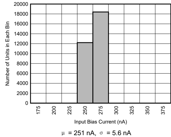
图 7-20. Input Bias Current Distribution
