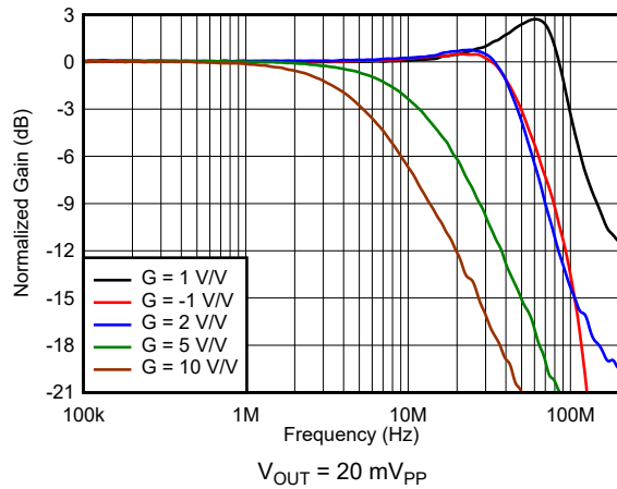
图 7-26. Small-Signal Frequency Response vs Gain
