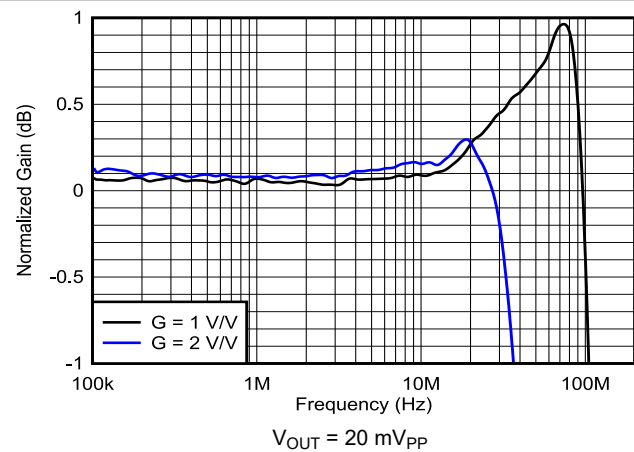
图 7-4. Small-Signal Response Flatness vs Gain
