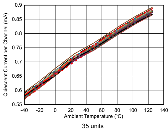
图 7-23. Quiescent Current vs Ambient Temperature
