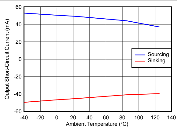
图 7-33. Output Short-Circuit Current vs Ambient Temperature
