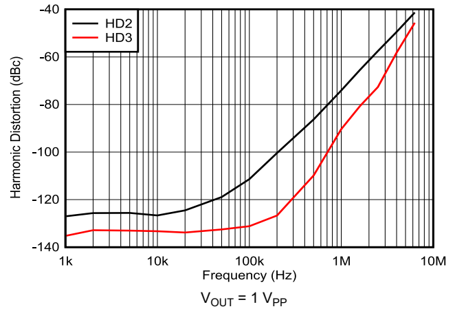
图 7-27. Harmonic Distortion vs Frequency
