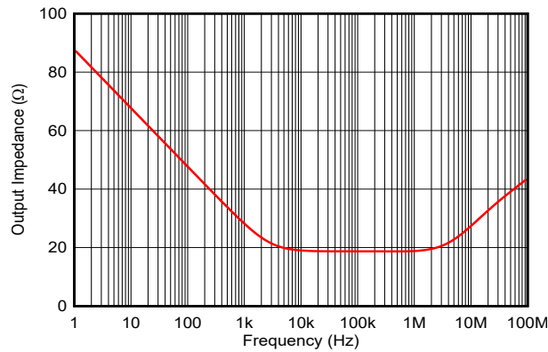
图 7-40. Open-Loop Output Impedance vs Frequency
