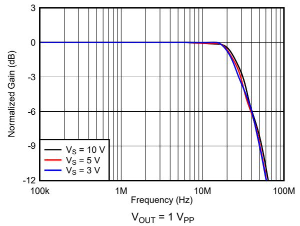
图 7-35. Frequency Response vs Supply Voltage
