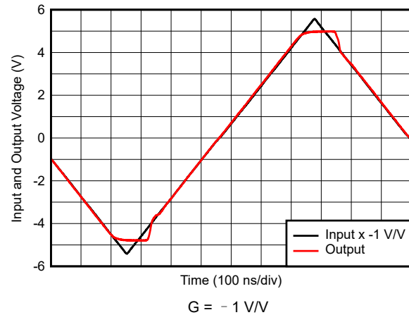
图 7-14. Output Overdrive Recovery
