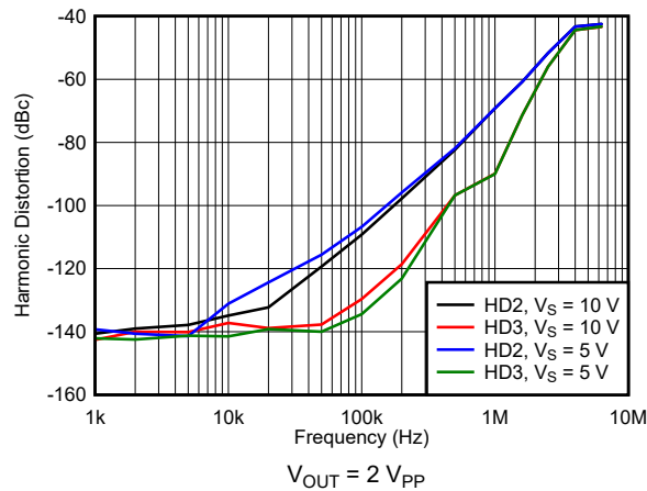
图 7-42. Harmonic Distortion vs Supply Voltage
