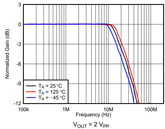
图 7-8. Frequency Response vs Ambient Temperature
