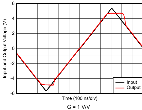
图 7-13. Input Overdrive Recovery
