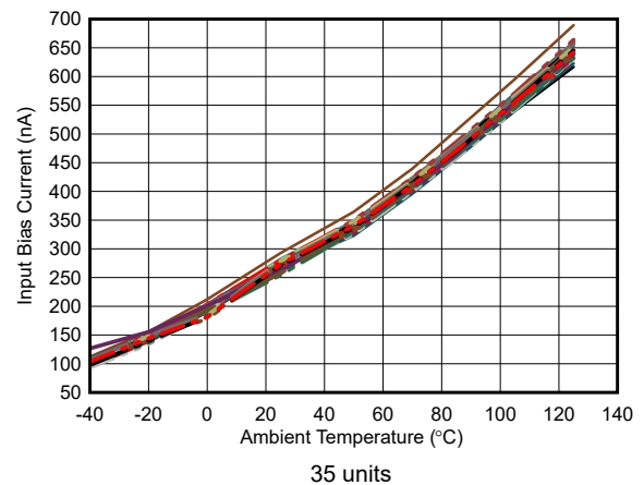
图 7-24. Input Bias Current vs Ambient Temperature
