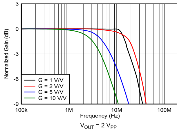
图 7-7. Large-Signal Frequency Response vs Gain
