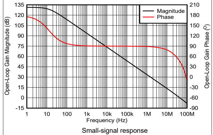
图 7-41. Open-Loop Gain and Phase vs Frequency
