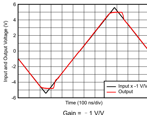
图 7-14. Output Overdrive Recovery
