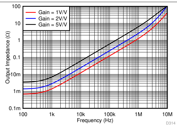
图 30. Closed-Loop Output Impedance vs Frequency
