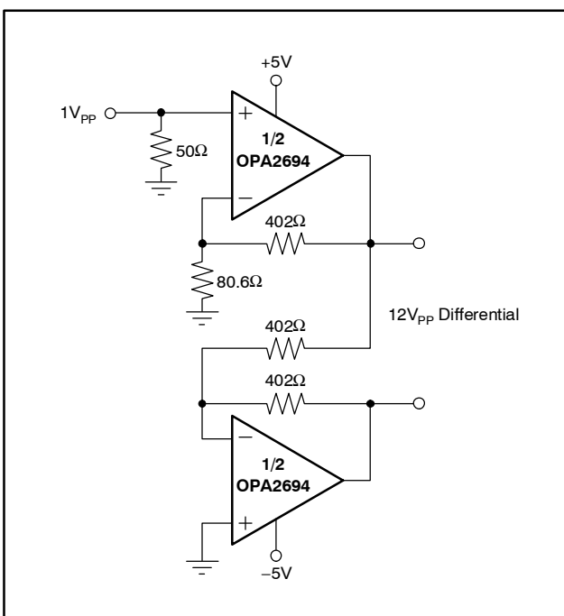
Figure 8. Single-to-Differential Conversion
