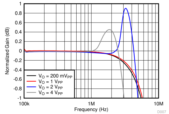
图 7-8. Large-Signal Response Flatness vs Frequency
