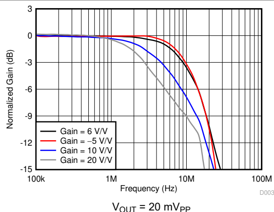
图 7-4. Small-Signal Frequency Response vs Gain
