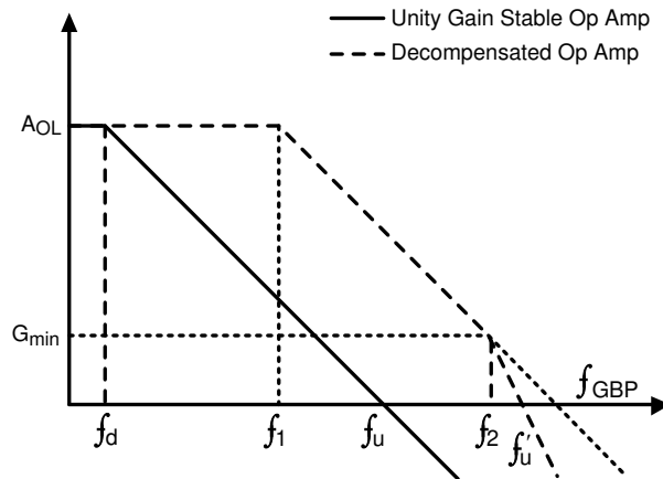
图 8-5. Gain vs Frequency Characteristics for a Unity-Gain Stable Op Amp and a Decompensated Op Amp
