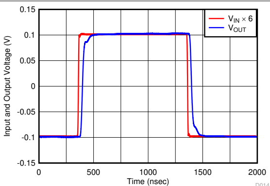
图 7-13. Output Overdrive Recovery
