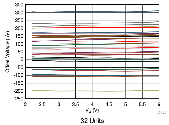
图 7-24. Input Offset vs Supply
