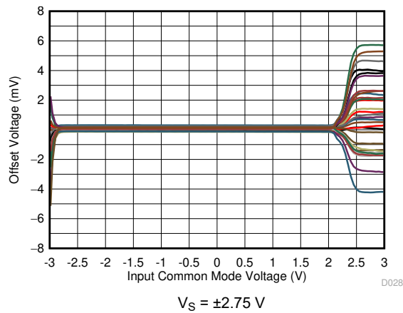
图 7-25. Input Offset vs Common Mode Voltage
