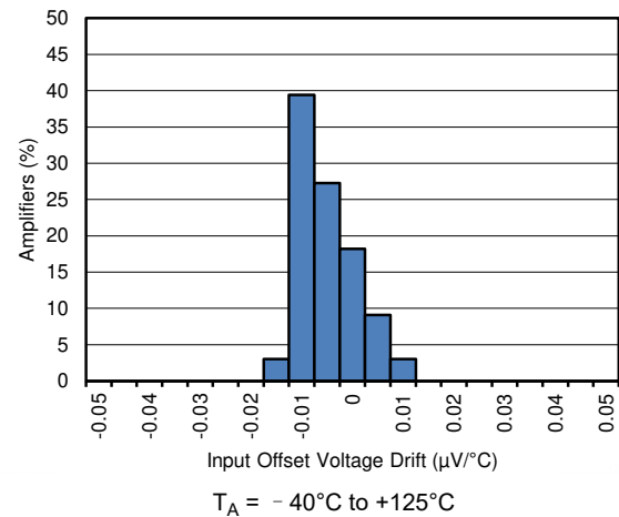
图 6-2. Offset Voltage Drift Distribution
