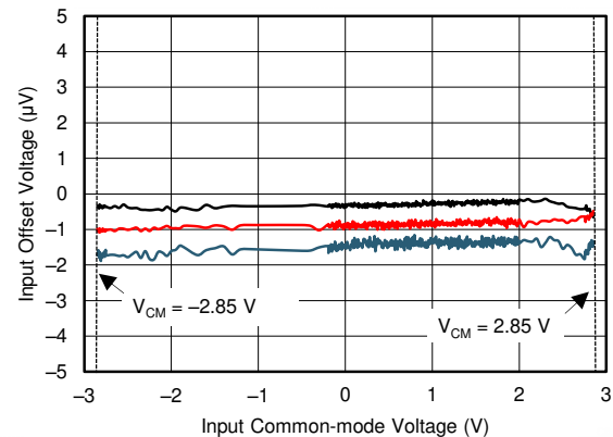
图 6-4. Offset Voltage vs Common-Mode Voltage
