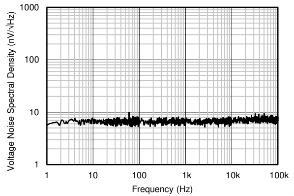
图 6-16. Input Voltage Noise Spectral Density vs Frequency
