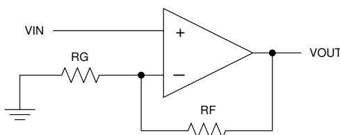
图 10-1. Schematic Representation
