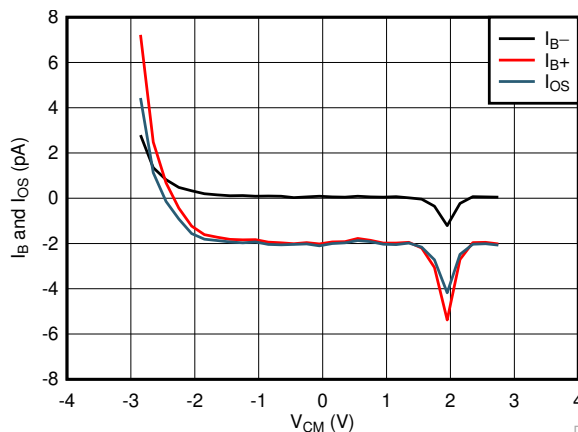
图 7-7. I_B and I_{OS} vs Common-Mode Voltage
