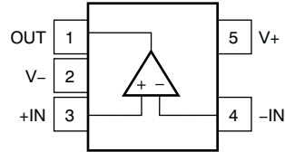
Pin Functions: OPA317-Q1
